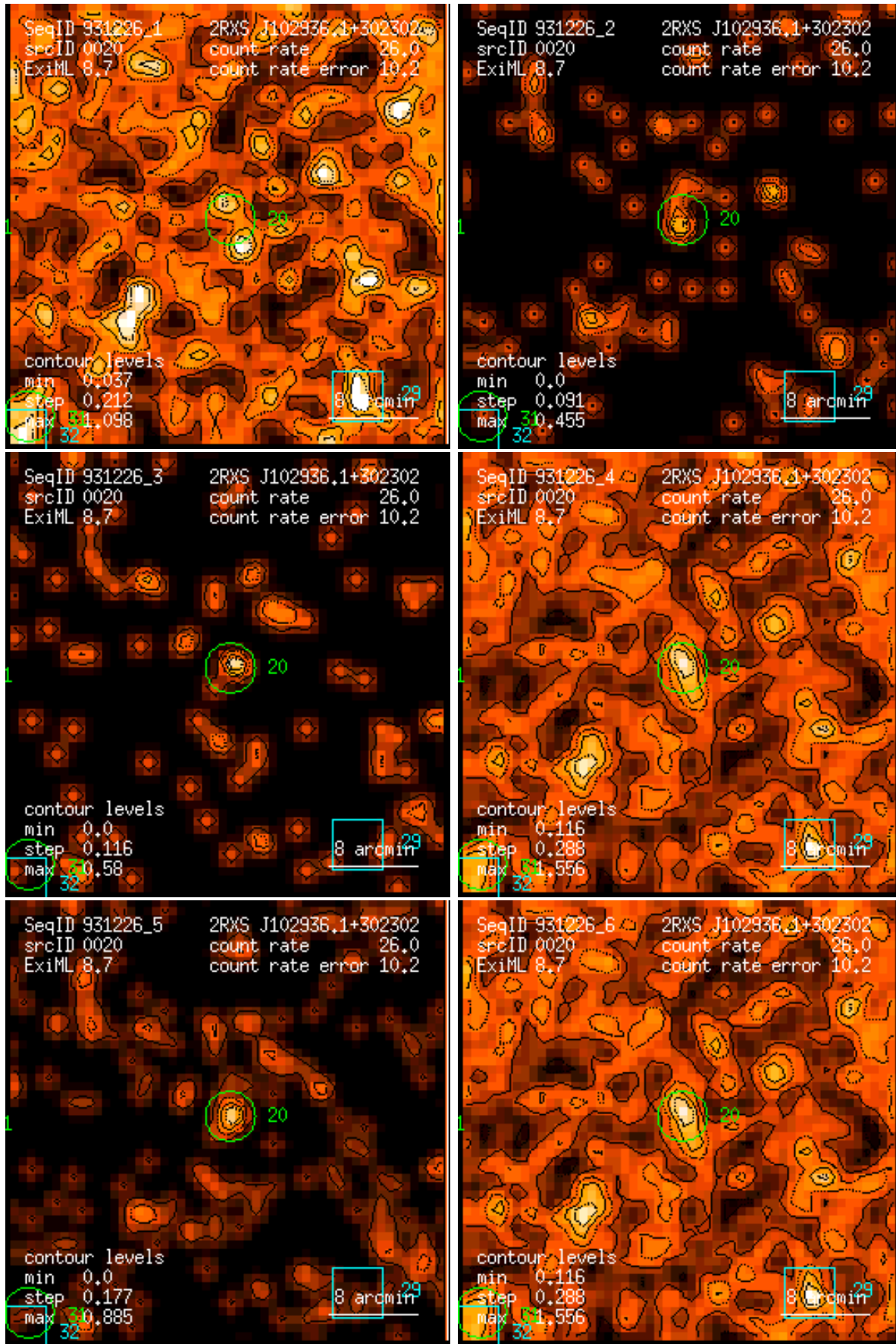
Figure 20: RASS 931226: detection 0020: band rate images, Gaussian filter: (1) PSPC channels 11 – 41, (2) 52 – 90, (3) 91 – 201, (4) 11 – 235, (5) 52 – 201, (6) 11 – 201. Broad band rates in counts/ks. Band rate contour levels in counts/ks/arcmin 2 .
