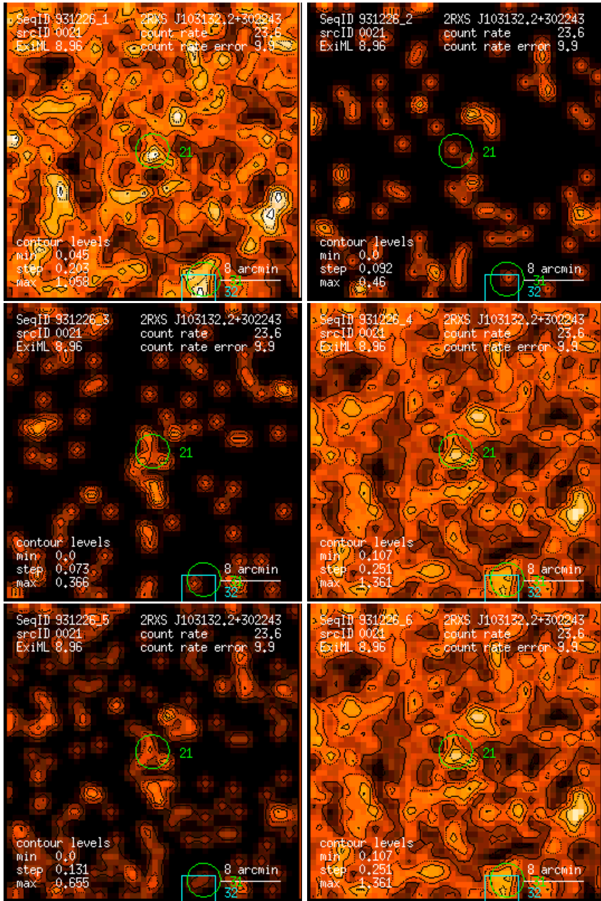
Figure 21: RASS 931226: detection 0021: band rate images, Gaussian filter: (1) PSPC channels 11 – 41, (2) 52 – 90, (3) 91 – 201, (4) 11 – 235, (5) 52 – 201, (6) 11 – 201. Broad band rates in counts/ks. Band rate contour levels in counts/ks/arcmin 2 .
