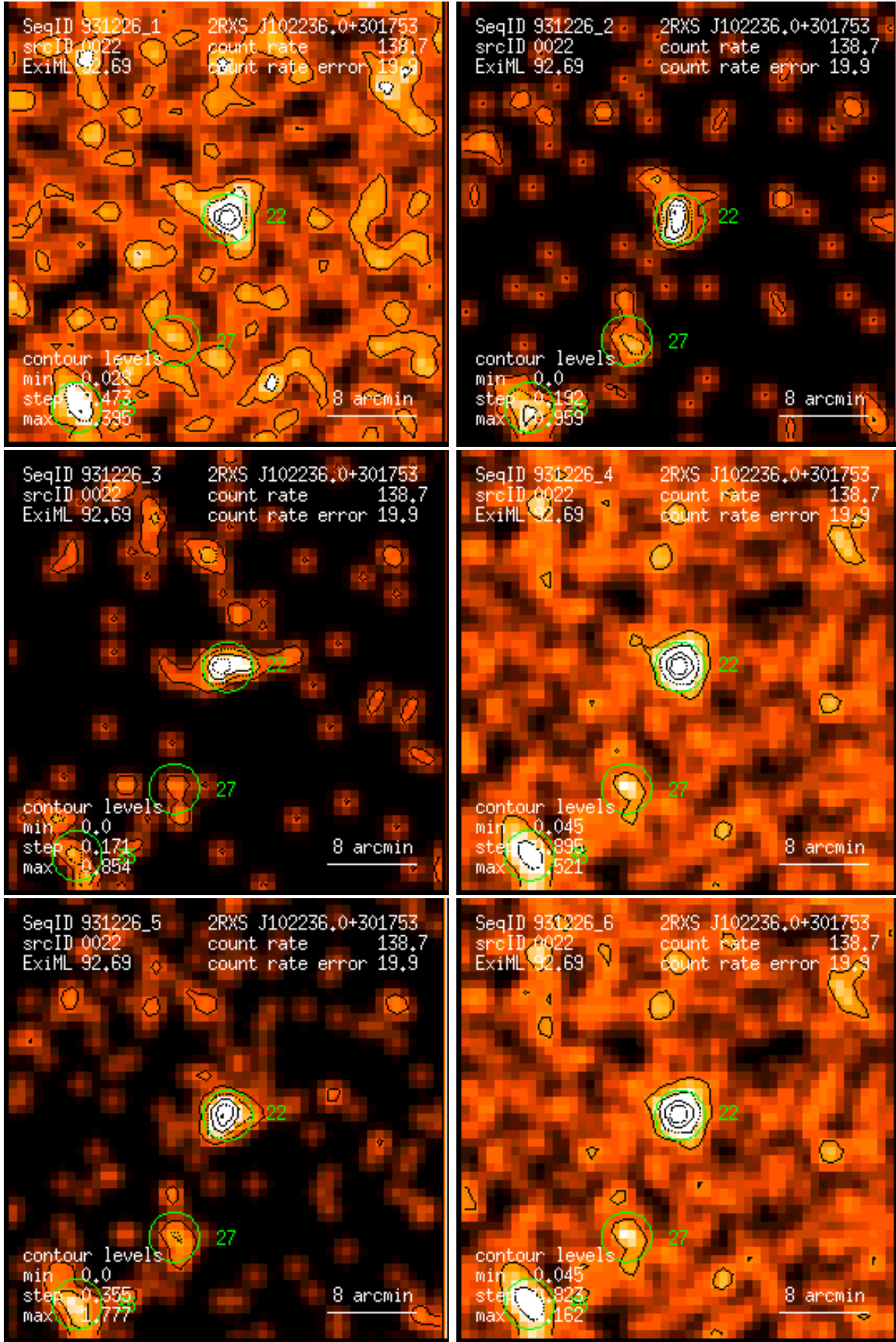
Figure 22: RASS 931226: detection 0022: band rate images, Gaussian filter: (1) PSPC channels 11 – 41, (2) 52 – 90, (3) 91 – 201, (4) 11 – 235, (5) 52 – 201, (6) 11 – 201. Broad band rates in counts/ks. Band rate contour levels in counts/ks/arcmin 2 .
