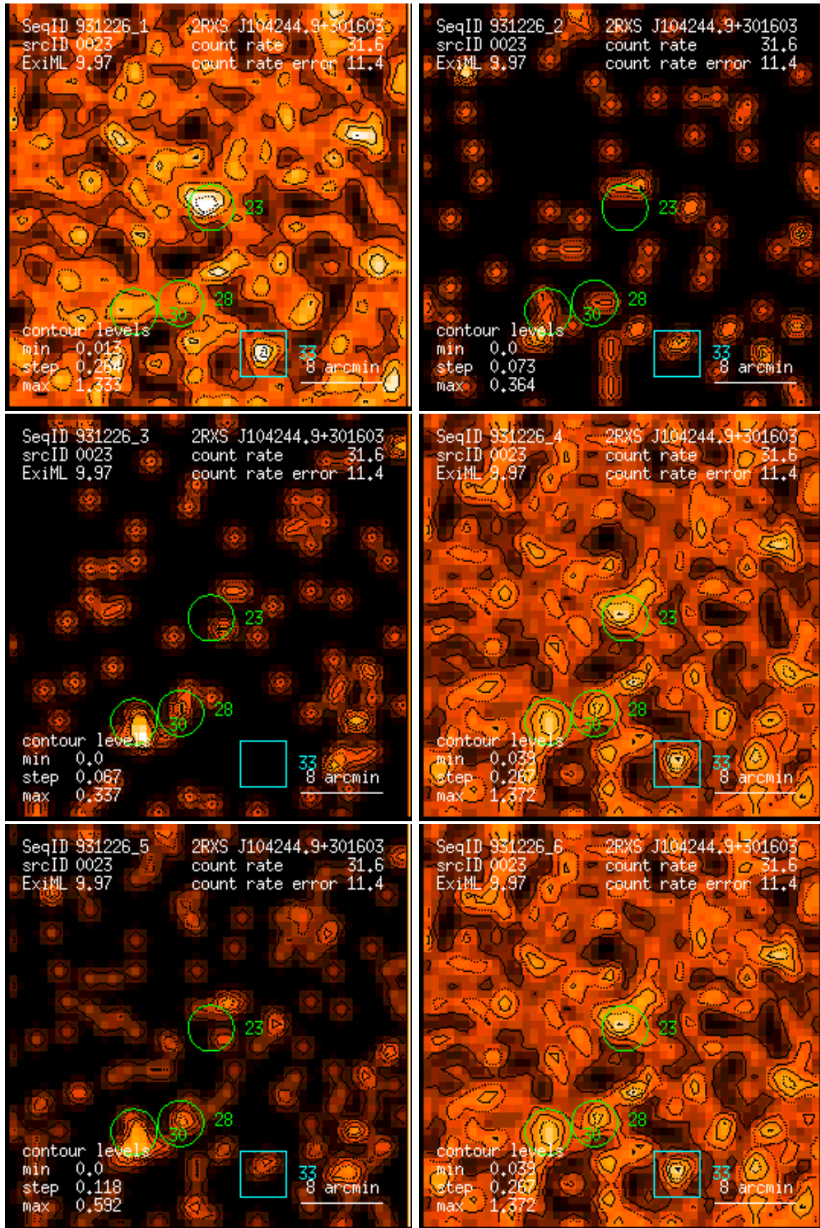
Figure 23: RASS 931226: detection 0023: band rate images, Gaussian filter: (1) PSPC channels 11 – 41, (2) 52 – 90, (3) 91 – 201, (4) 11 – 235, (5) 52 – 201, (6) 11 – 201. Broad band rates in counts/ks. Band rate contour levels in counts/ks/arcmin 2 .
