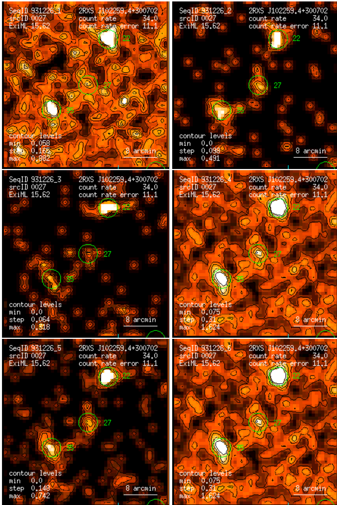
Figure 27: RASS 931226: detection 0027: band rate images, Gaussian filter: (1) PSPC channels 11 – 41, (2) 52 – 90, (3) 91 – 201, (4) 11 – 235, (5) 52 – 201, (6) 11 – 201. Broad band rates in counts/ks. Band rate contour levels in counts/ks/arcmin 2 .
