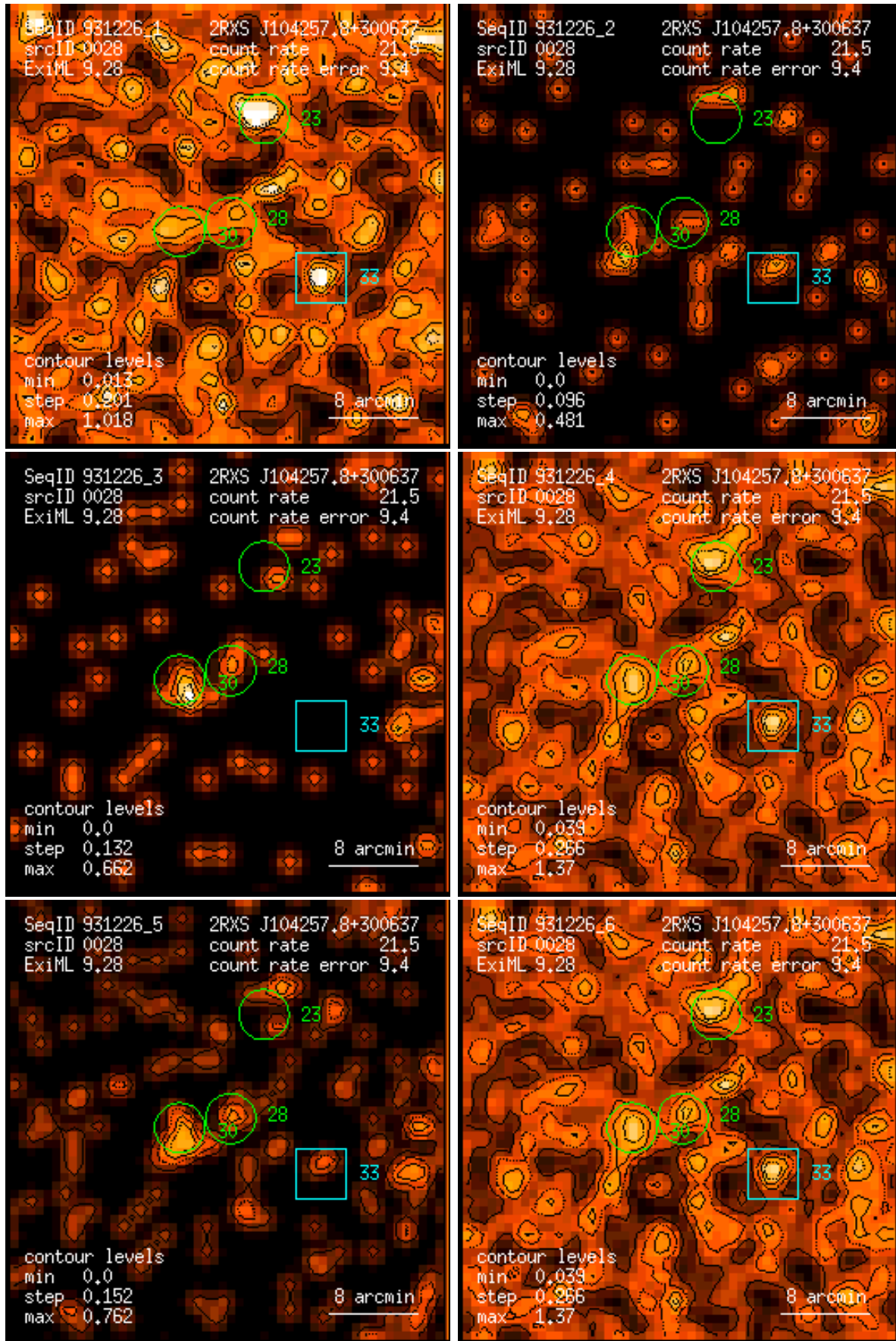
Figure 28: RASS 931226: detection 0028: band rate images, Gaussian filter: (1) PSPC channels 11 – 41, (2) 52 – 90, (3) 91 – 201, (4) 11 – 235, (5) 52 – 201, (6) 11 – 201. Broad band rates in counts/ks. Band rate contour levels in counts/ks/arcmin 2 .
