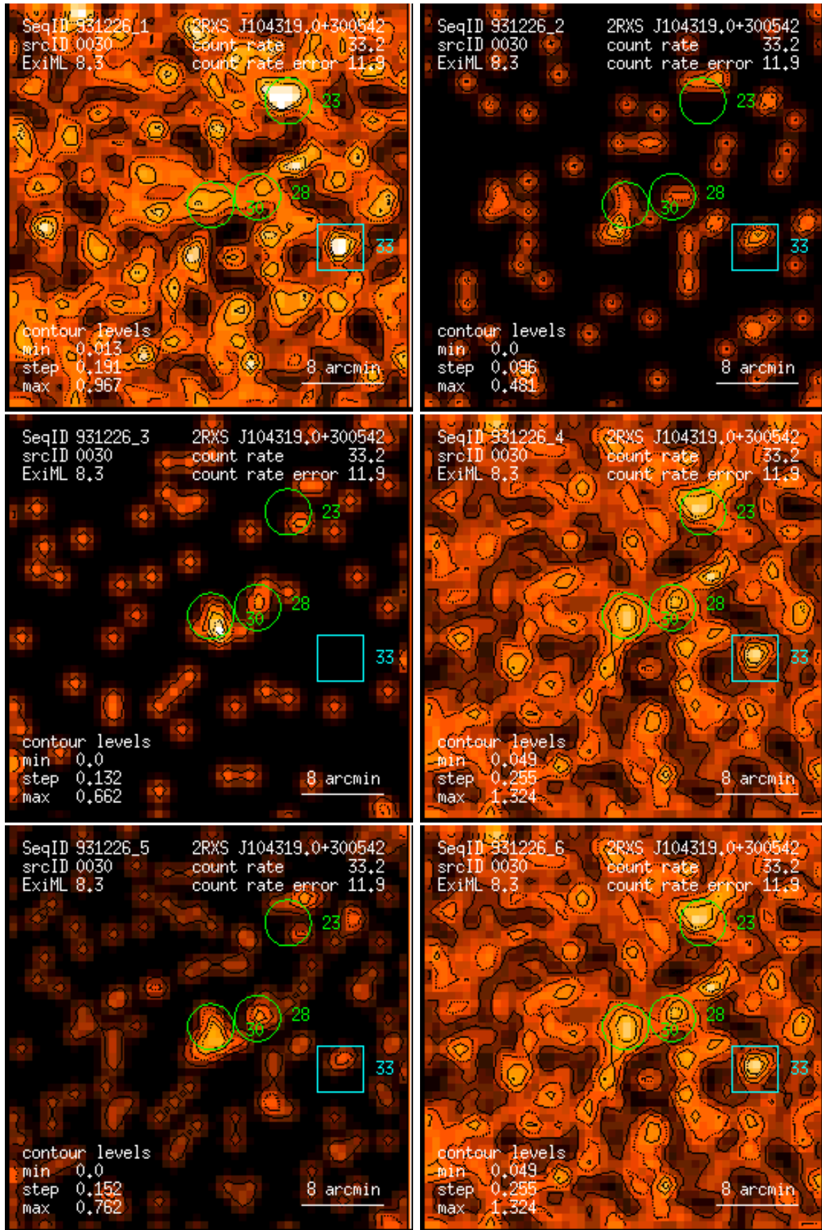
Figure 30: RASS 931226: detection 0030: band rate images, Gaussian filter: (1) PSPC channels 11 – 41, (2) 52 – 90, (3) 91 – 201, (4) 11 – 235, (5) 52 – 201, (6) 11 – 201. Broad band rates in counts/ks. Band rate contour levels in counts/ks/arcmin 2 .
