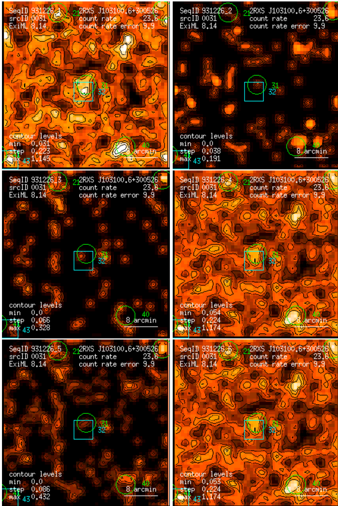
Figure 31: RASS 931226: detection 0031: band rate images, Gaussian filter: (1) PSPC channels 11 – 41, (2) 52 – 90, (3) 91 – 201, (4) 11 – 235, (5) 52 – 201, (6) 11 – 201. Broad band rates in counts/ks. Band rate contour levels in counts/ks/arcmin 2 .
