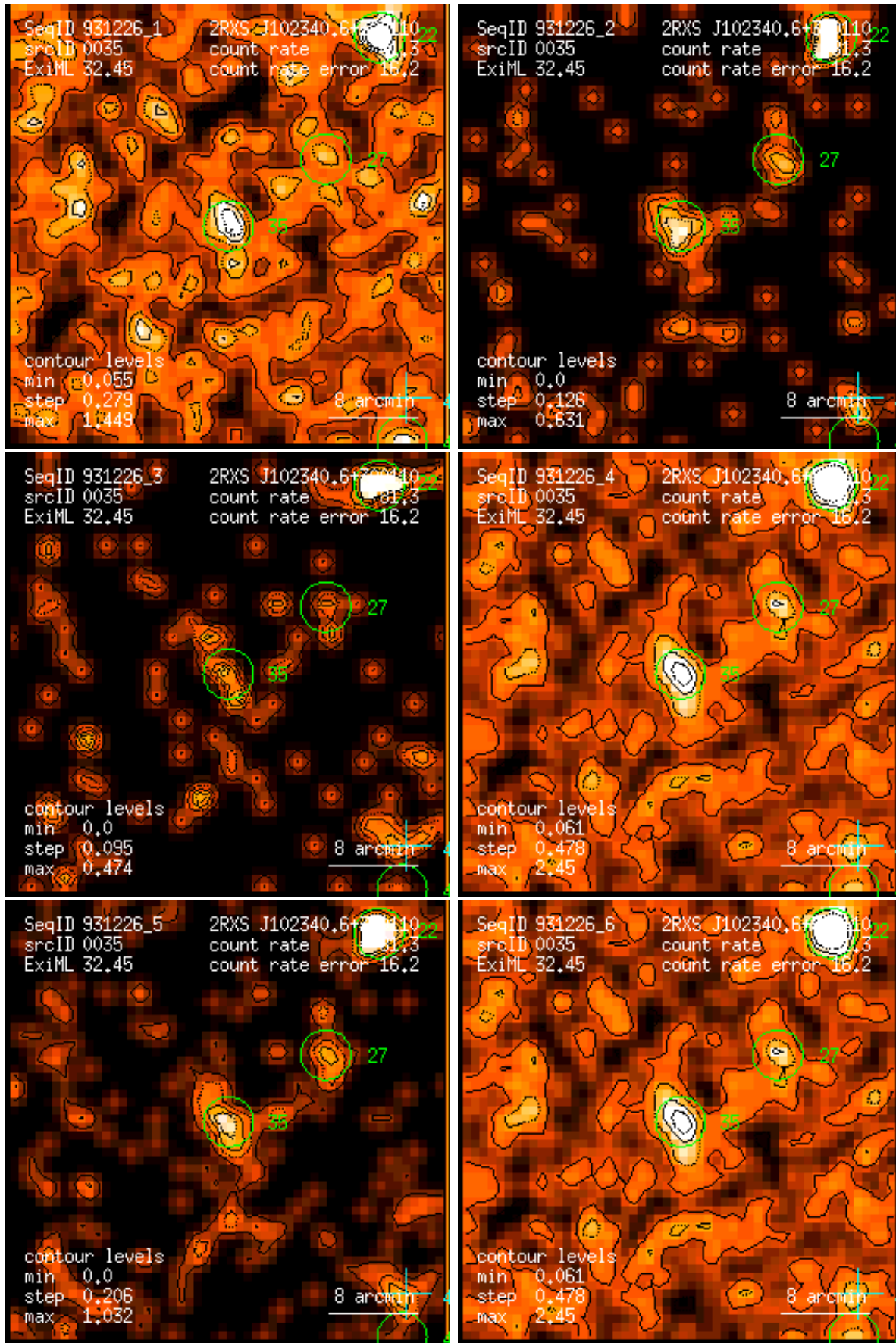
Figure 35: RASS 931226: detection 0035: band rate images, Gaussian filter: (1) PSPC channels 11 – 41, (2) 52 – 90, (3) 91 – 201, (4) 11 – 235, (5) 52 – 201, (6) 11 – 201. Broad band rates in counts/ks. Band rate contour levels in counts/ks/arcmin 2 .
