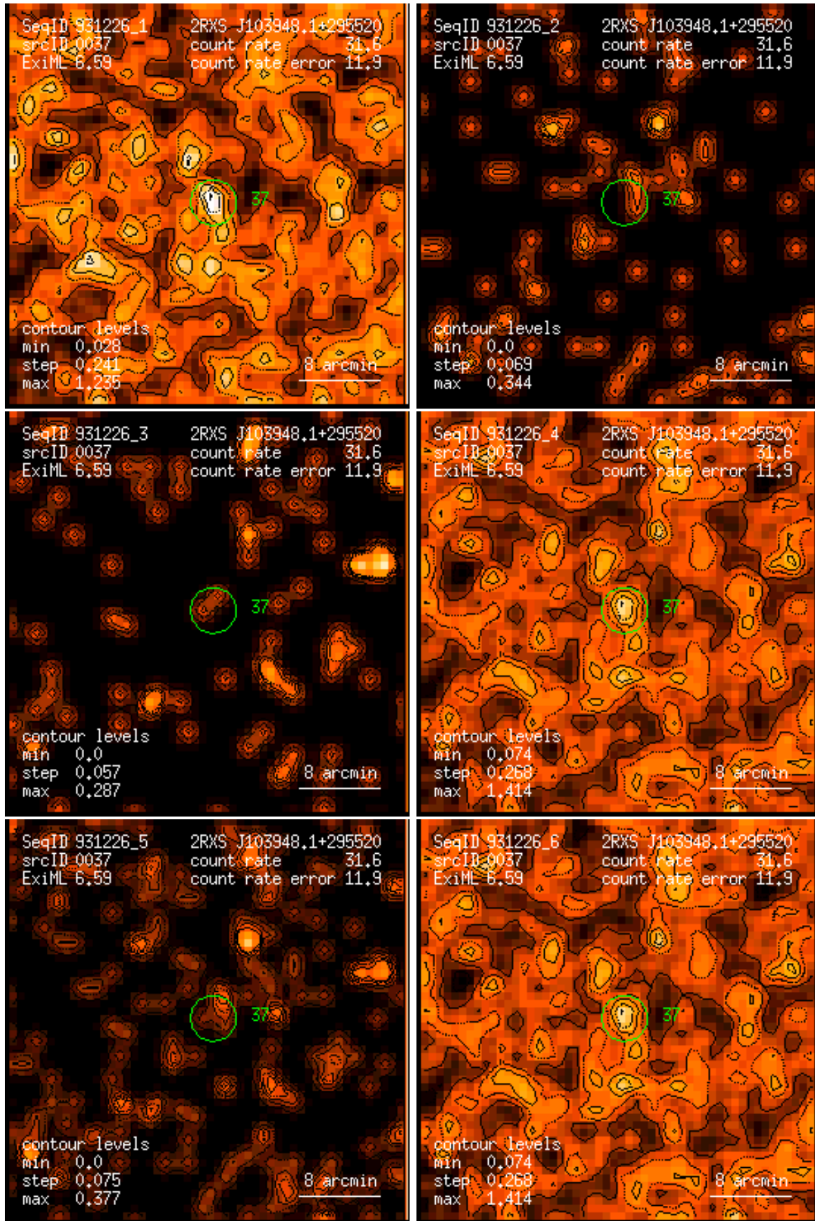
Figure 37: RASS 931226: detection 0037: band rate images, Gaussian filter: (1) PSPC channels 11 – 41, (2) 52 – 90, (3) 91 – 201, (4) 11 – 235, (5) 52 – 201, (6) 11 – 201. Broad band rates in counts/ks. Band rate contour levels in counts/ks/arcmin 2 .
