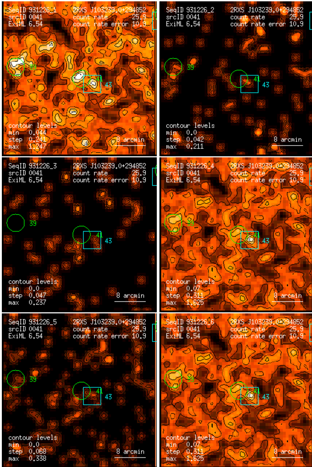
Figure 41: RASS 931226: detection 0041: band rate images, Gaussian filter: (1) PSPC channels 11 – 41, (2) 52 – 90, (3) 91 – 201, (4) 11 – 235, (5) 52 – 201, (6) 11 – 201. Broad band rates in counts/ks. Band rate contour levels in counts/ks/arcmin 2 .
