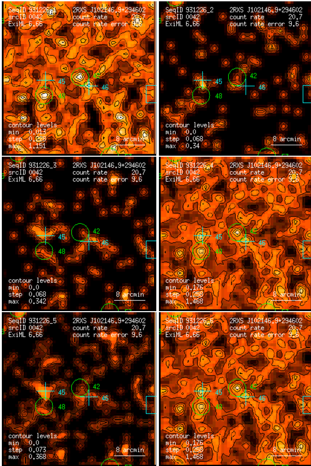
Figure 42: RASS 931226: detection 0042: band rate images, Gaussian filter: (1) PSPC channels 11 – 41, (2) 52 – 90, (3) 91 – 201, (4) 11 – 235, (5) 52 – 201, (6) 11 – 201. Broad band rates in counts/ks. Band rate contour levels in counts/ks/arcmin 2 .
