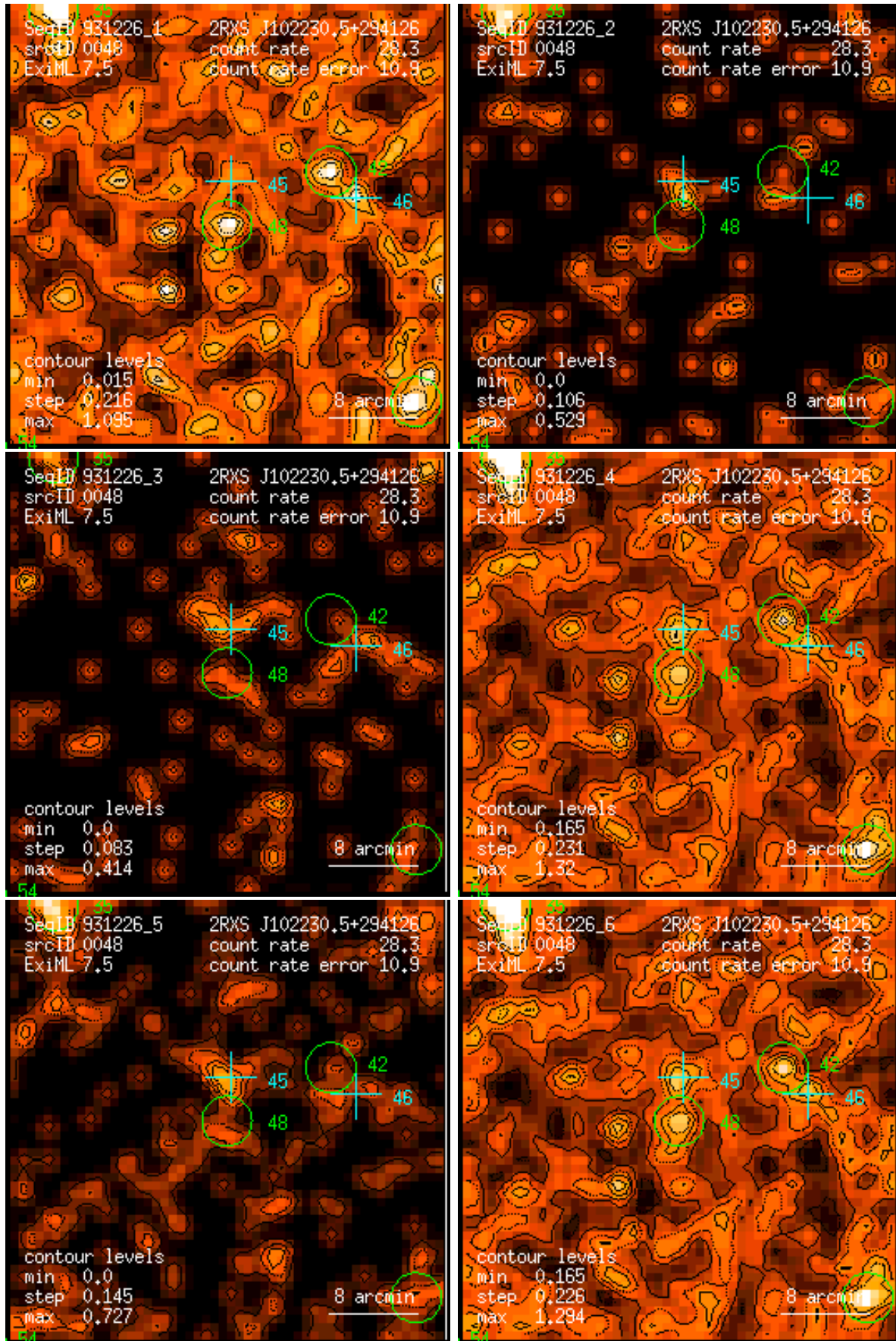
Figure 48: RASS 931226: detection 0048: band rate images, Gaussian filter: (1) PSPC channels 11 – 41, (2) 52 – 90, (3) 91 – 201, (4) 11 – 235, (5) 52 – 201, (6) 11 – 201. Broad band rates in counts/ks. Band rate contour levels in counts/ks/arcmin 2 .
