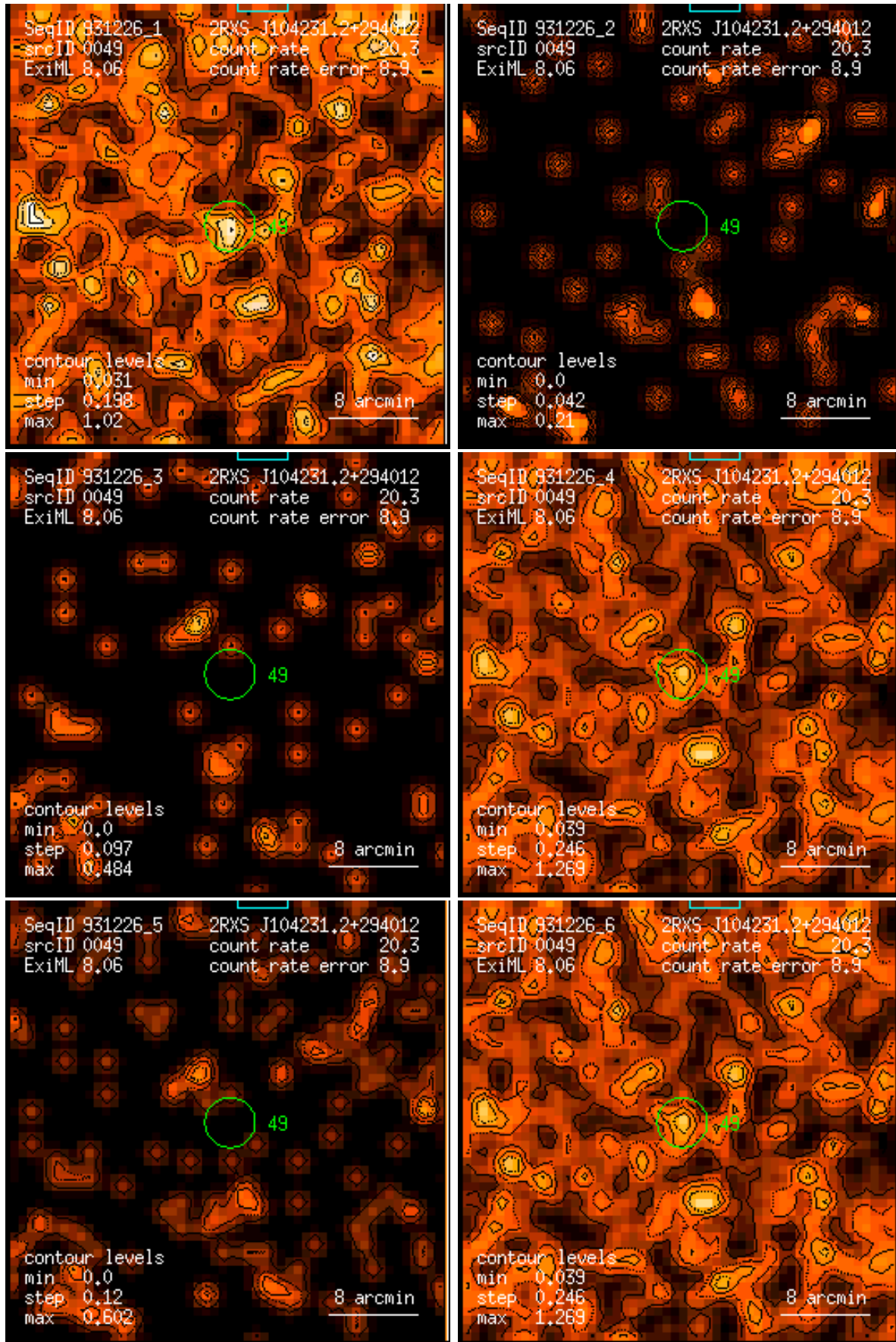
Figure 49: RASS 931226: detection 0049: band rate images, Gaussian filter: (1) PSPC channels 11 – 41, (2) 52 – 90, (3) 91 – 201, (4) 11 – 235, (5) 52 – 201, (6) 11 – 201. Broad band rates in counts/ks. Band rate contour levels in counts/ks/arcmin 2 .
