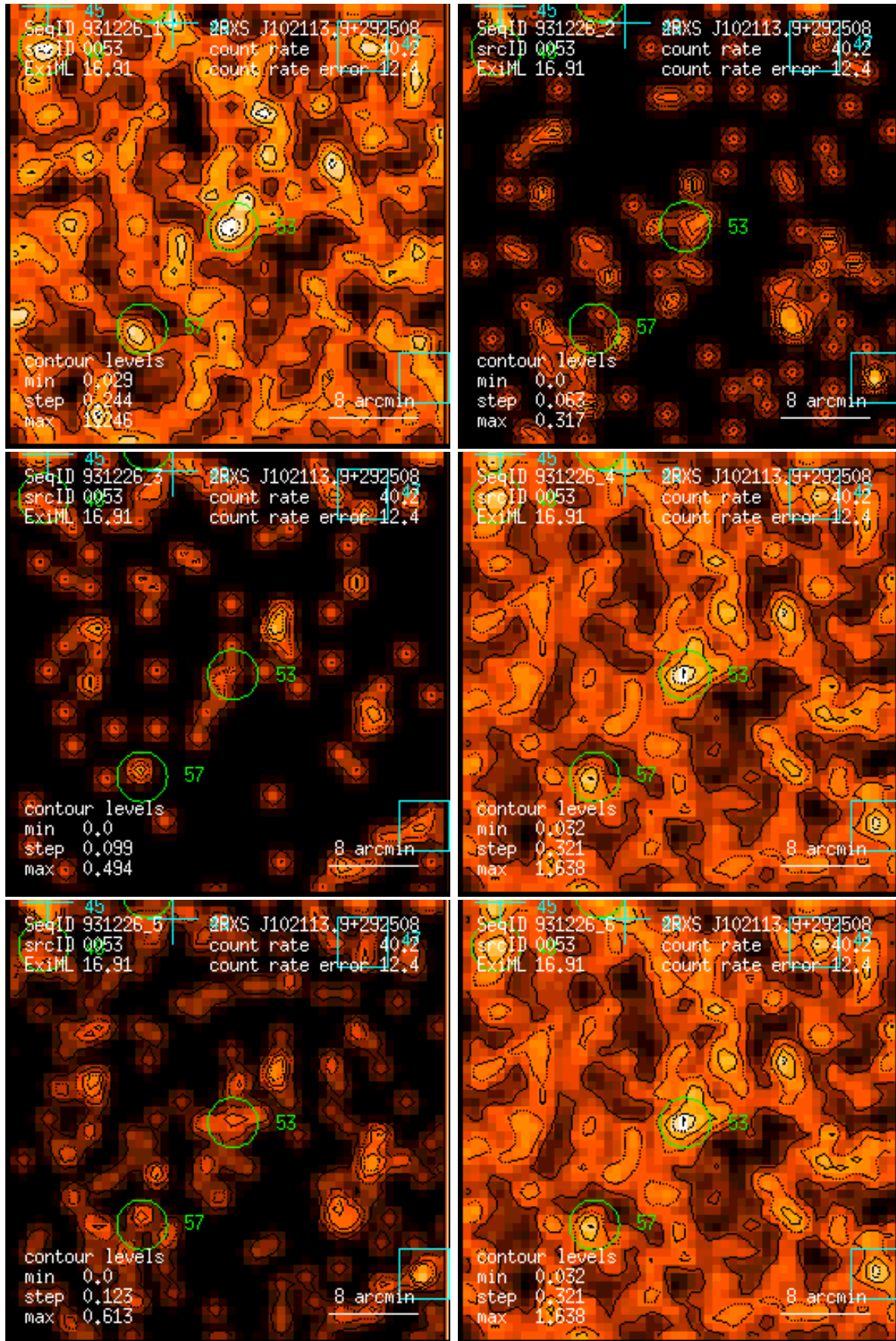
Figure 53: RASS 931226: detection 0053: band rate images, Gaussian filter: (1) PSPC channels 11 – 41, (2) 52 – 90, (3) 91 – 201, (4) 11 – 235, (5) 52 – 201, (6) 11 – 201. Broad band rates in counts/ks. Band rate contour levels in counts/ks/arcmin 2 .
