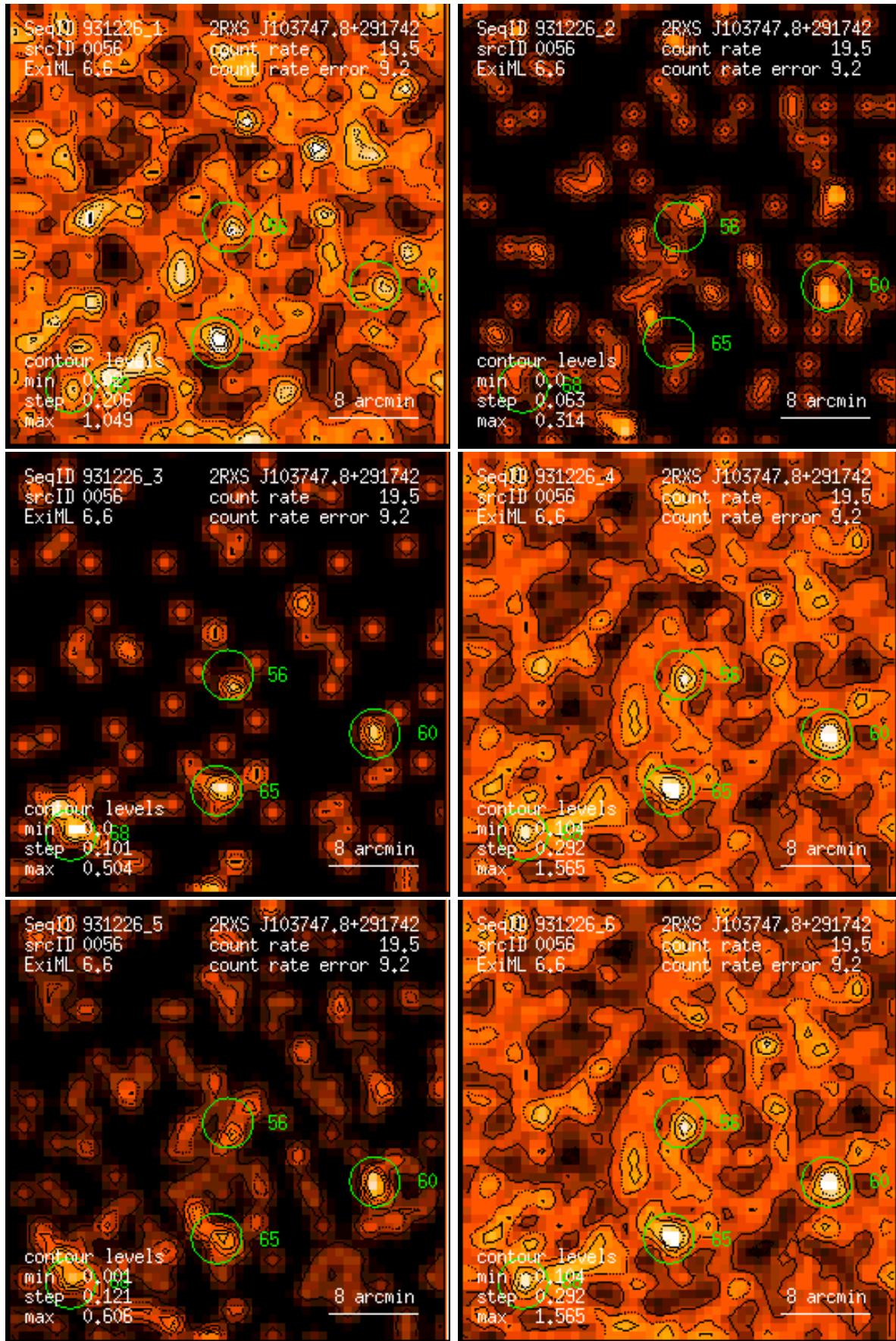
Figure 56: RASS 931226: detection 0056: band rate images, Gaussian filter: (1) PSPC channels 11 – 41, (2) 52 – 90, (3) 91 – 201, (4) 11 – 235, (5) 52 – 201, (6) 11 – 201. Broad band rates in counts/ks. Band rate contour levels in counts/ks/arcmin 2 .
