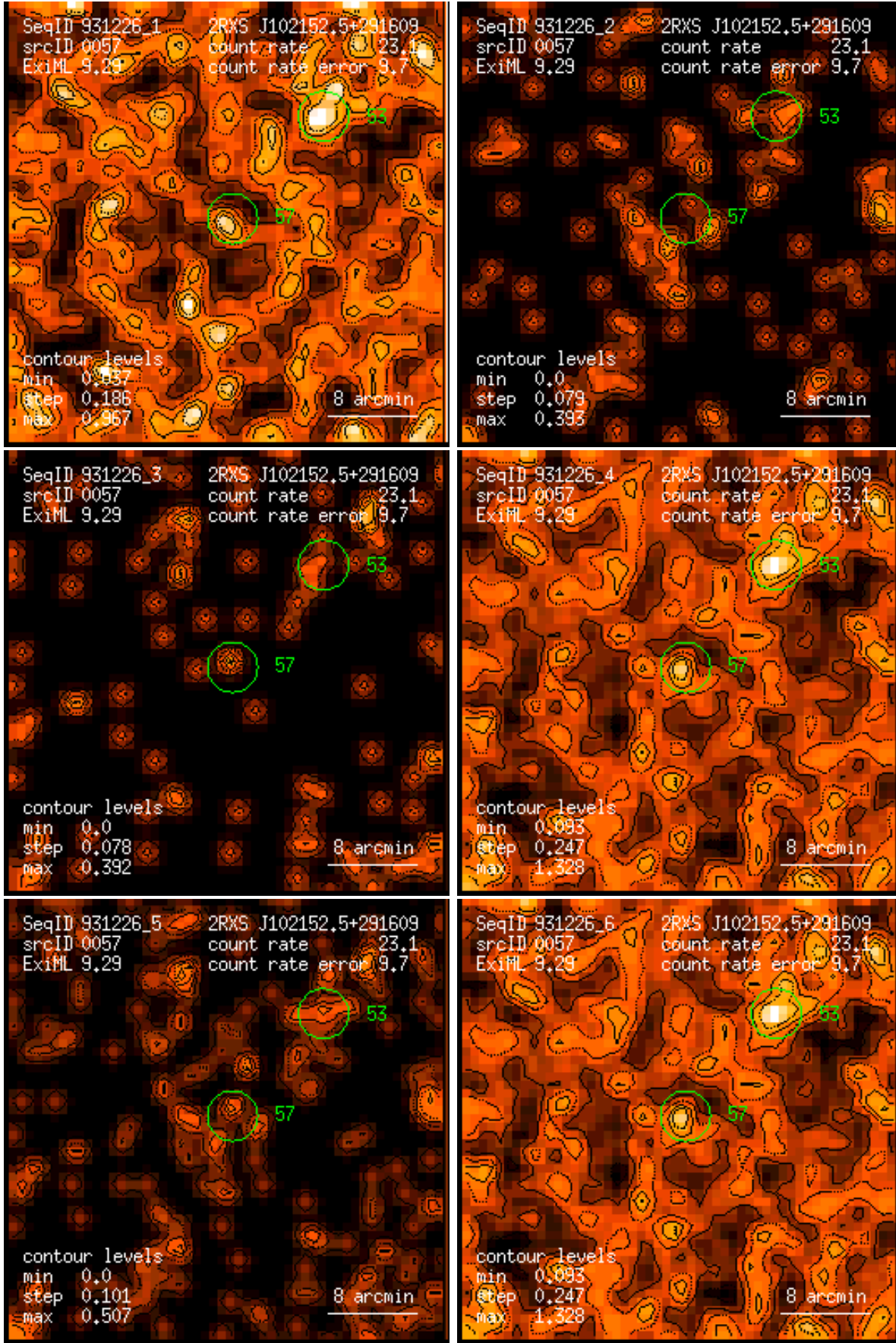
Figure 57: RASS 931226: detection 0057: band rate images, Gaussian filter: (1) PSPC channels 11 – 41, (2) 52 – 90, (3) 91 – 201, (4) 11 – 235, (5) 52 – 201, (6) 11 – 201. Broad band rates in counts/ks. Band rate contour levels in counts/ks/arcmin 2 .
