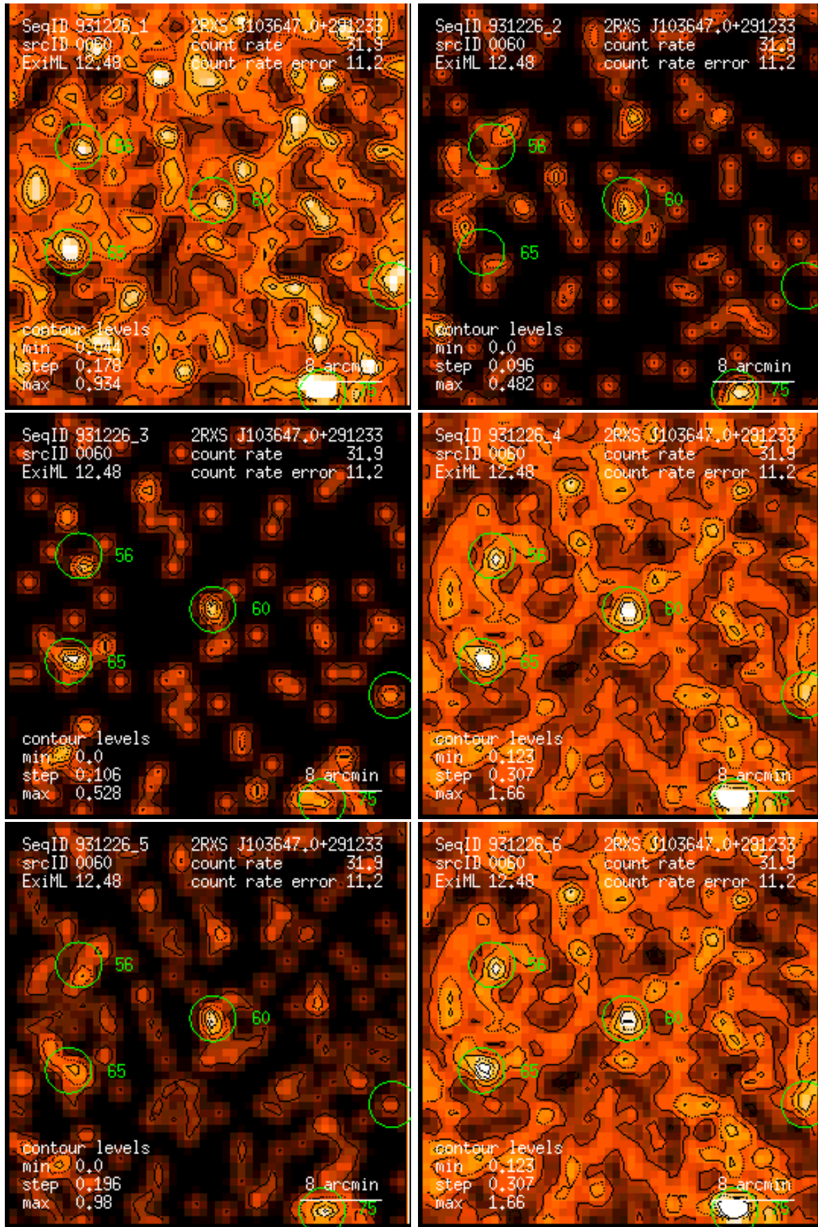
Figure 60: RASS 931226: detection 0060: band rate images, Gaussian filter: (1) PSPC channels 11 – 41, (2) 52 – 90, (3) 91 – 201, (4) 11 – 235, (5) 52 – 201, (6) 11 – 201. Broad band rates in counts/ks. Band rate contour levels in counts/ks/arcmin 2 .
