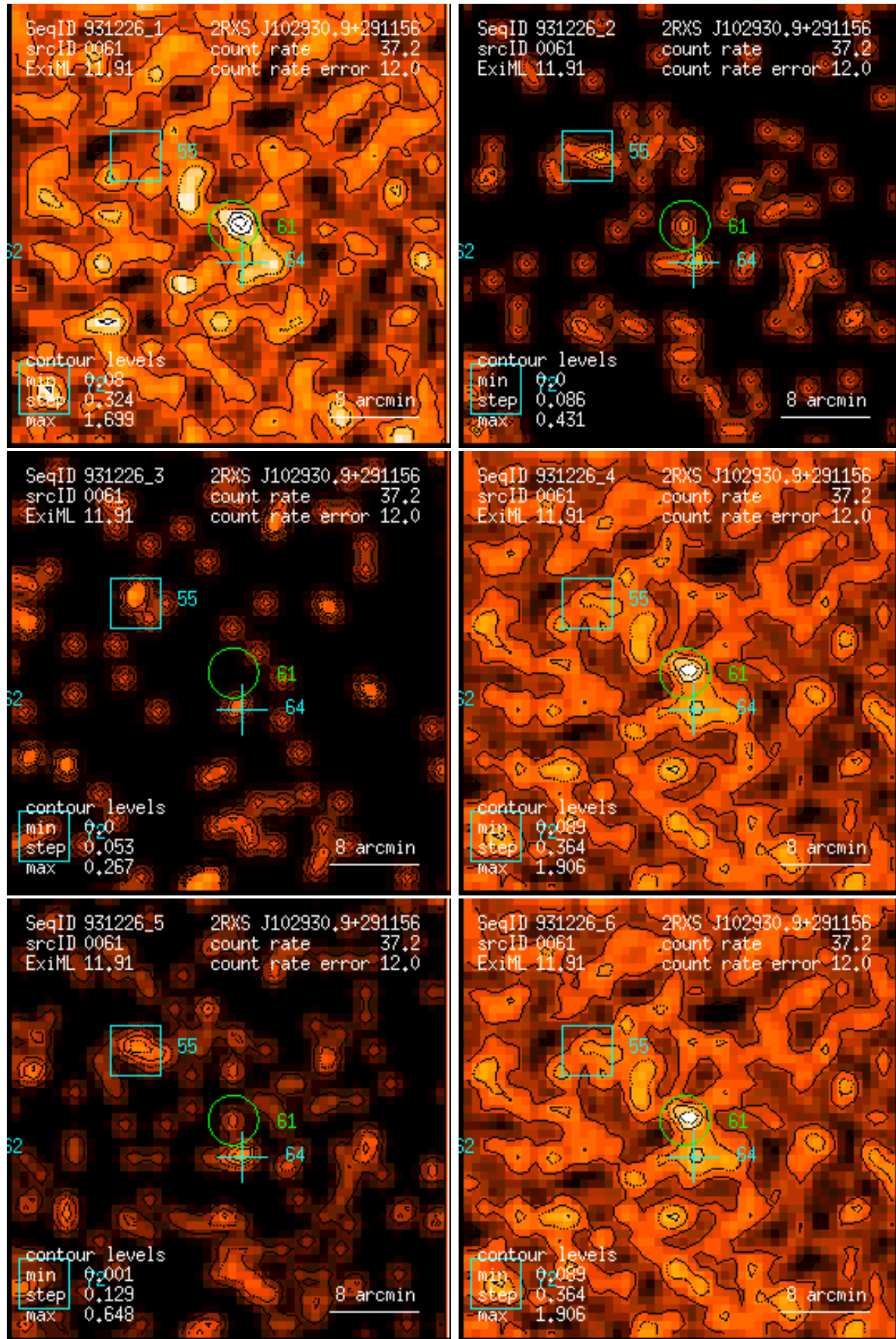
Figure 61: RASS 931226: detection 0061: band rate images, Gaussian filter: (1) PSPC channels 11 – 41, (2) 52 – 90, (3) 91 – 201, (4) 11 – 235, (5) 52 – 201, (6) 11 – 201. Broad band rates in counts/ks. Band rate contour levels in counts/ks/arcmin 2 .
