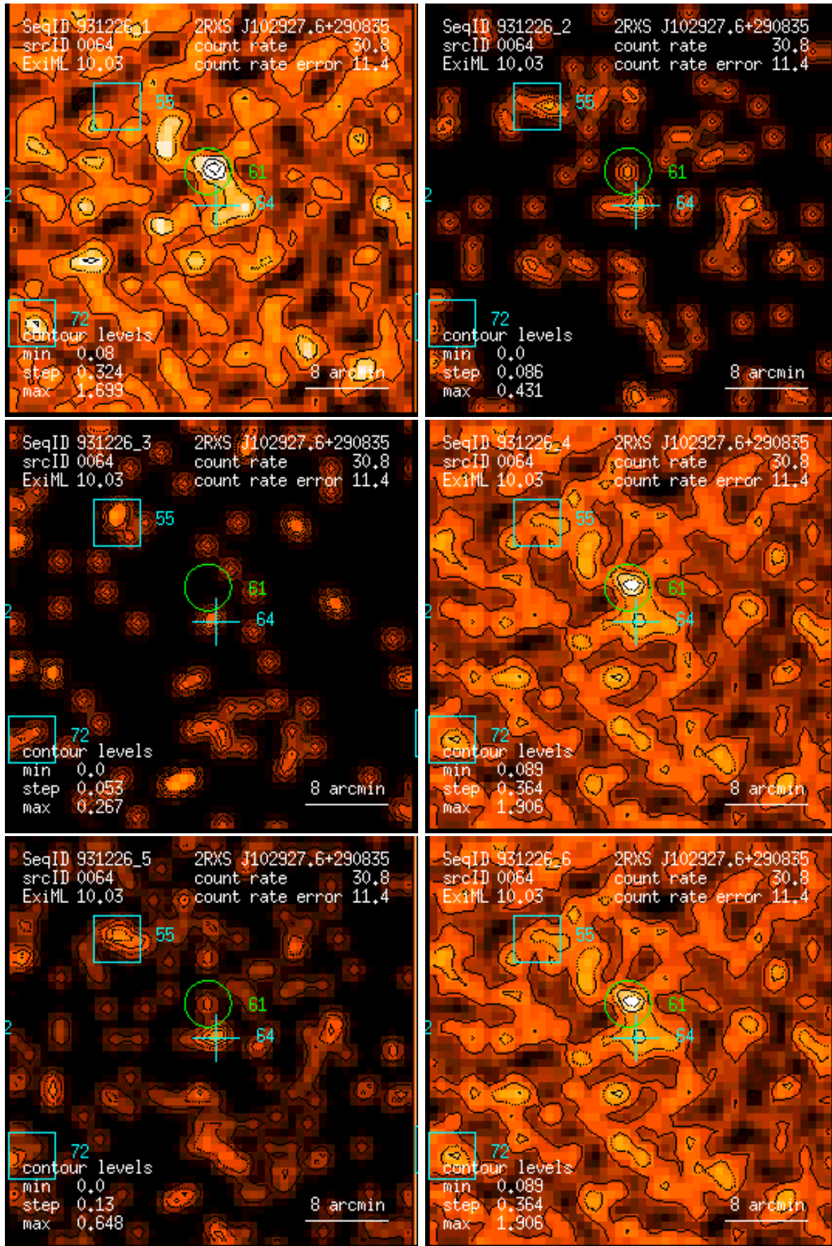
Figure 64: RASS 931226: detection 0064: band rate images, Gaussian filter: (1) PSPC channels 11 – 41, (2) 52 – 90, (3) 91 – 201, (4) 11 – 235, (5) 52 – 201, (6) 11 – 201. Broad band rates in counts/ks. Band rate contour levels in counts/ks/arcmin 2 .
