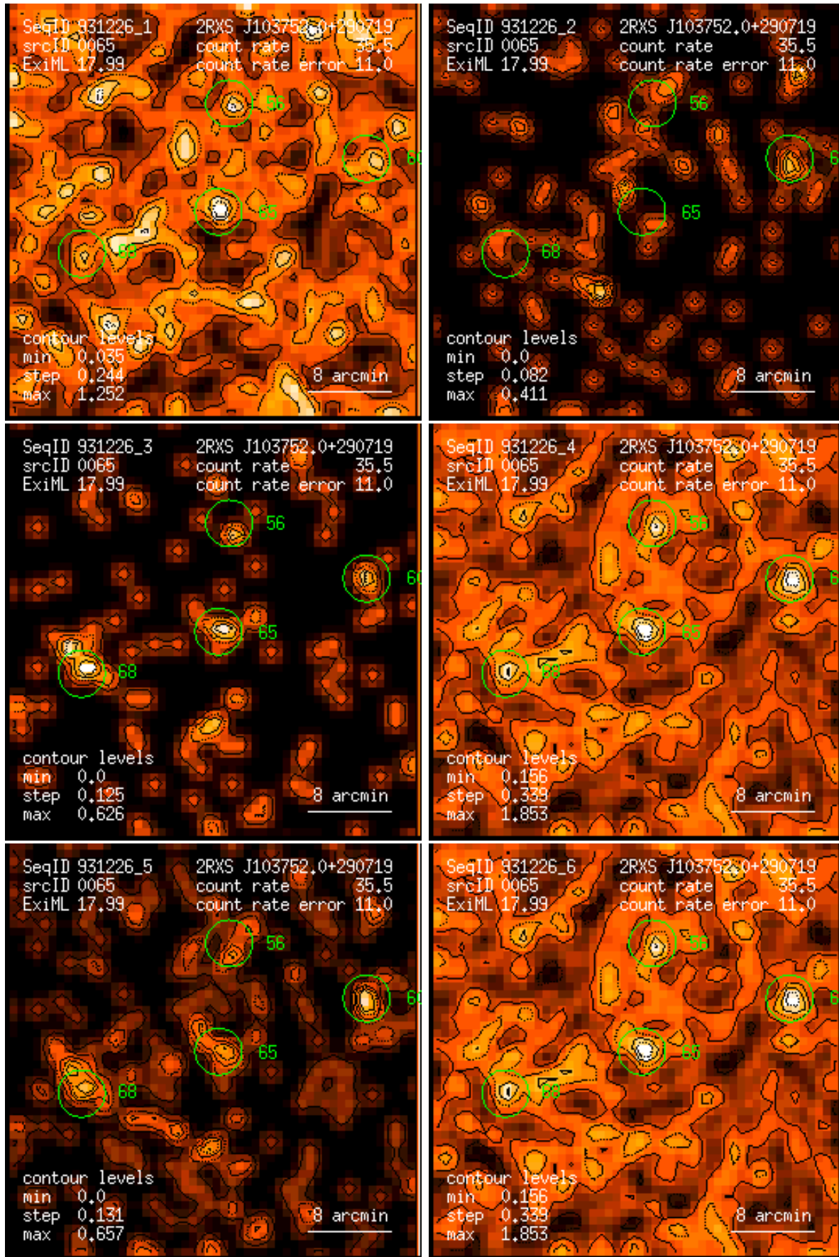
Figure 65: RASS 931226: detection 0065: band rate images, Gaussian filter: (1) PSPC channels 11 – 41, (2) 52 – 90, (3) 91 – 201, (4) 11 – 235, (5) 52 – 201, (6) 11 – 201. Broad band rates in counts/ks. Band rate contour levels in counts/ks/arcmin 2 .
