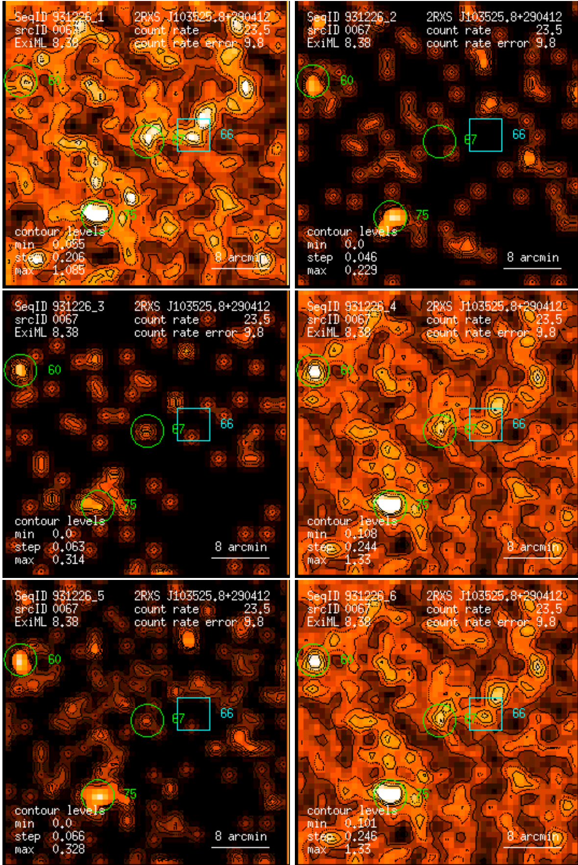
Figure 67: RASS 931226: detection 0067: band rate images, Gaussian filter: (1) PSPC channels 11 – 41, (2) 52 – 90, (3) 91 – 201, (4) 11 – 235, (5) 52 – 201, (6) 11 – 201. Broad band rates in counts/ks. Band rate contour levels in counts/ks/arcmin 2 .
