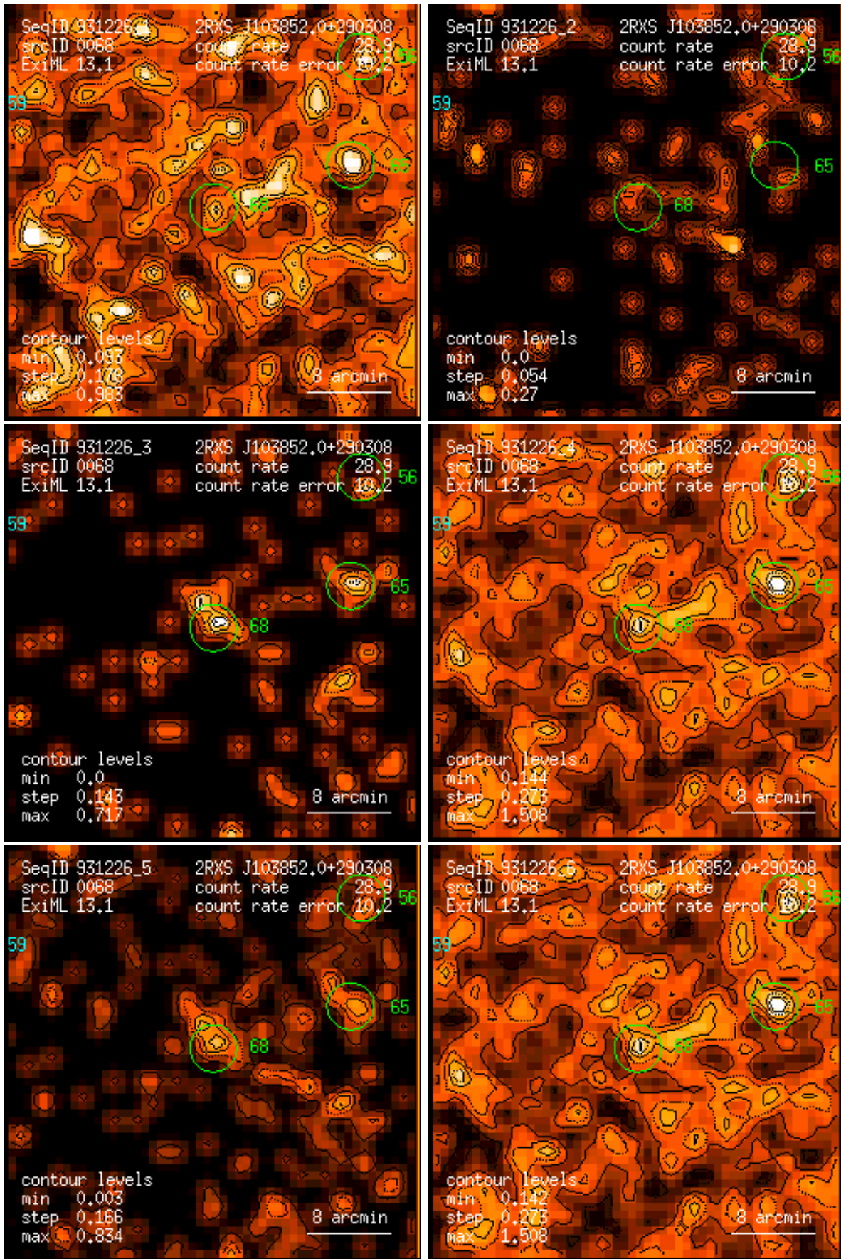
Figure 68: RASS 931226: detection 0068: band rate images, Gaussian filter: (1) PSPC channels 11 – 41, (2) 52 – 90, (3) 91 – 201, (4) 11 – 235, (5) 52 – 201, (6) 11 – 201. Broad band rates in counts/ks. Band rate contour levels in counts/ks/arcmin 2 .
