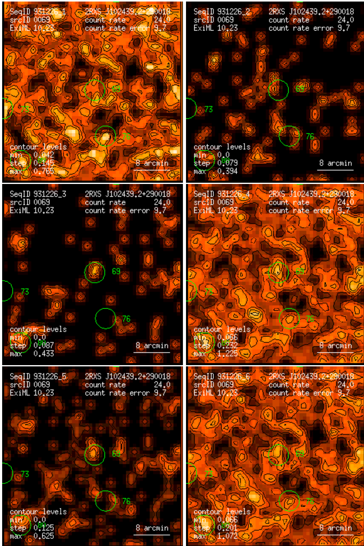
Figure 69: RASS 931226: detection 0069: band rate images, Gaussian filter: (1) PSPC channels 11 – 41, (2) 52 – 90, (3) 91 – 201, (4) 11 – 235, (5) 52 – 201, (6) 11 – 201. Broad band rates in counts/ks. Band rate contour levels in counts/ks/arcmin 2 .
