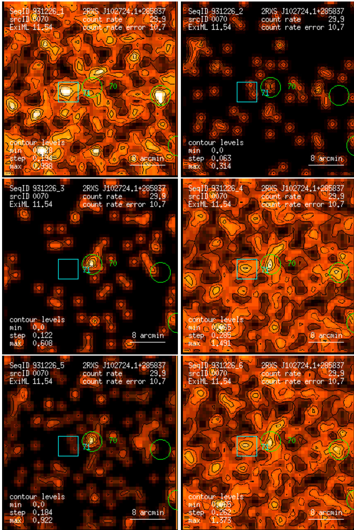
Figure 70: RASS 931226: detection 0070: band rate images, Gaussian filter: (1) PSPC channels 11 – 41, (2) 52 – 90, (3) 91 – 201, (4) 11 – 235, (5) 52 – 201, (6) 11 – 201. Broad band rates in counts/ks. Band rate contour levels in counts/ks/arcmin 2 .
