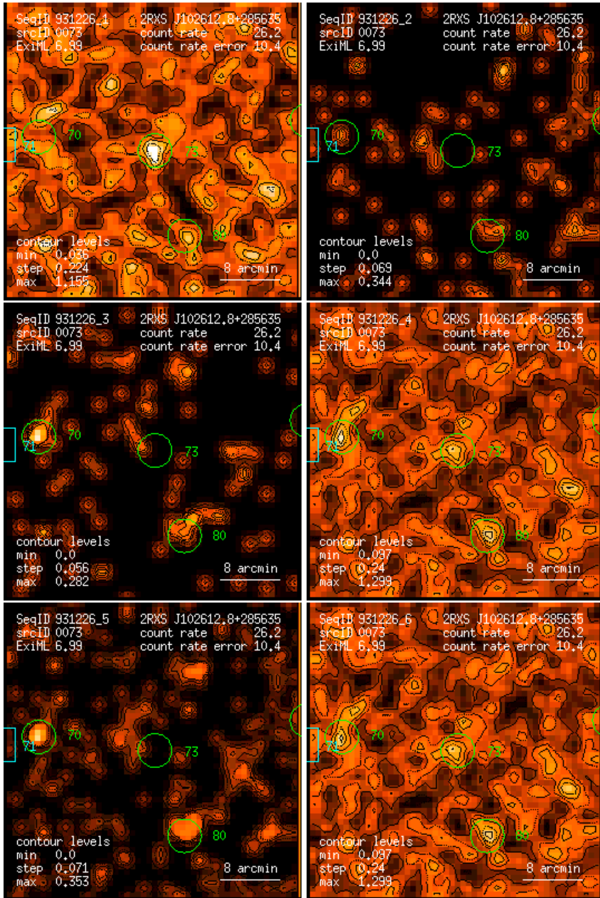
Figure 73: RASS 931226: detection 0073: band rate images, Gaussian filter: (1) PSPC channels 11 – 41, (2) 52 – 90, (3) 91 – 201, (4) 11 – 235, (5) 52 – 201, (6) 11 – 201. Broad band rates in counts/ks. Band rate contour levels in counts/ks/arcmin 2 .
