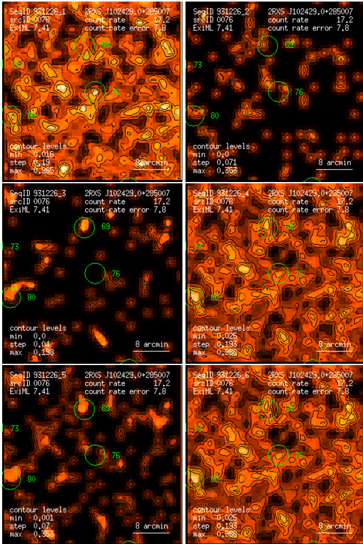
Figure 76: RASS 931226: detection 0076: band rate images, Gaussian filter: (1) PSPC channels 11 – 41, (2) 52 – 90, (3) 91 – 201, (4) 11 – 235, (5) 52 – 201, (6) 11 – 201. Broad band rates in counts/ks. Band rate contour levels in counts/ks/arcmin 2 .
