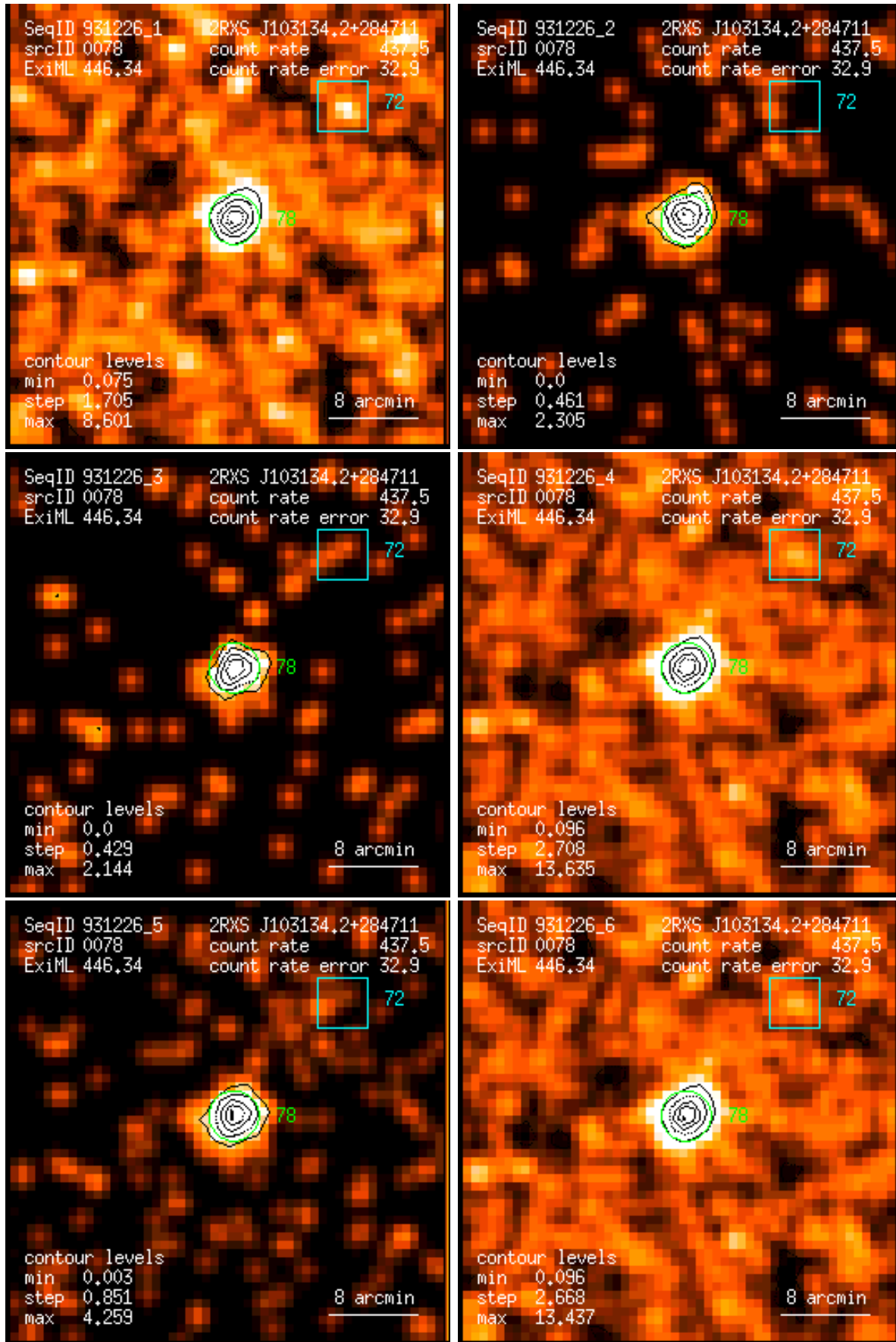
Figure 78: RASS 931226: detection 0078: band rate images, Gaussian filter: (1) PSPC channels 11 – 41, (2) 52 – 90, (3) 91 – 201, (4) 11 – 235, (5) 52 – 201, (6) 11 – 201. Broad band rates in counts/ks. Band rate contour levels in counts/ks/arcmin 2 .
