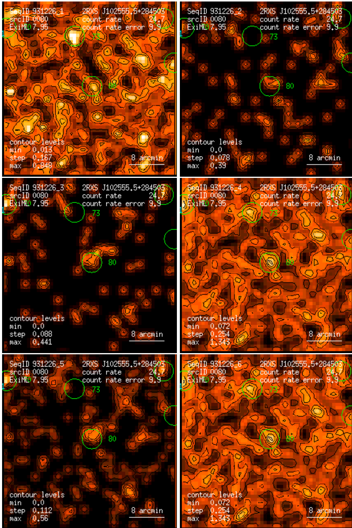
Figure 80: RASS 931226: detection 0080: band rate images, Gaussian filter: (1) PSPC channels 11 – 41, (2) 52 – 90, (3) 91 – 201, (4) 11 – 235, (5) 52 – 201, (6) 11 – 201. Broad band rates in counts/ks. Band rate contour levels in counts/ks/arcmin 2 .
