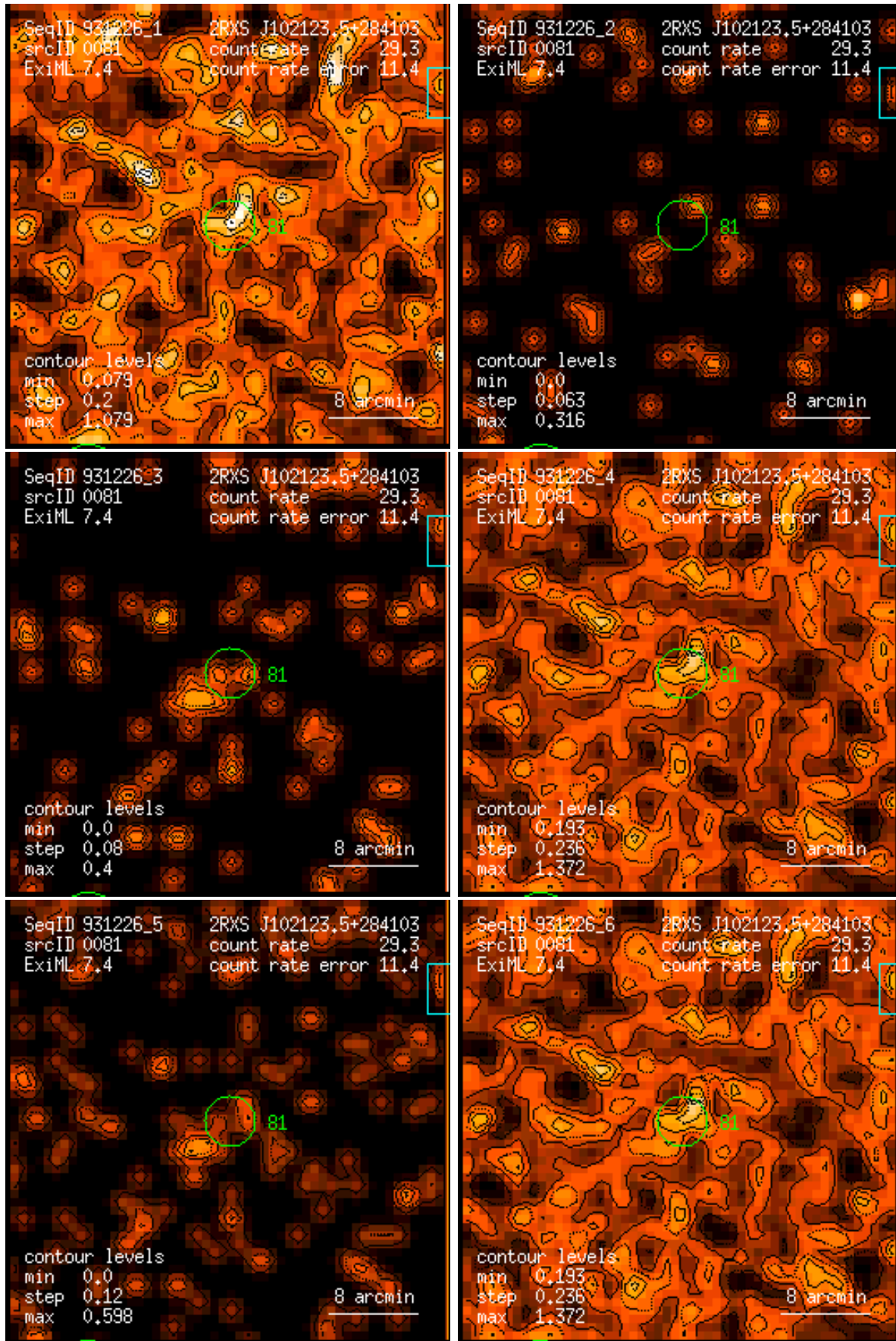
Figure 81: RASS 931226: detection 0081: band rate images, Gaussian filter: (1) PSPC channels 11 – 41, (2) 52 – 90, (3) 91 – 201, (4) 11 – 235, (5) 52 – 201, (6) 11 – 201. Broad band rates in counts/ks. Band rate contour levels in counts/ks/arcmin 2 .
