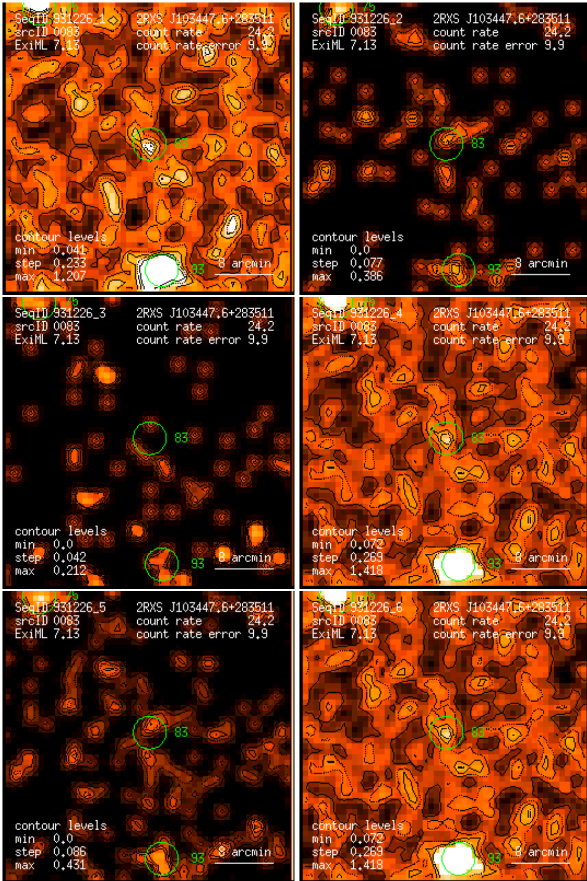
Figure 83: RASS 931226: detection 0083: band rate images, Gaussian filter: (1) PSPC channels 11 – 41, (2) 52 – 90, (3) 91 – 201, (4) 11 – 235, (5) 52 – 201, (6) 11 – 201. Broad band rates in counts/ks. Band rate contour levels in counts/ks/arcmin 2 .
