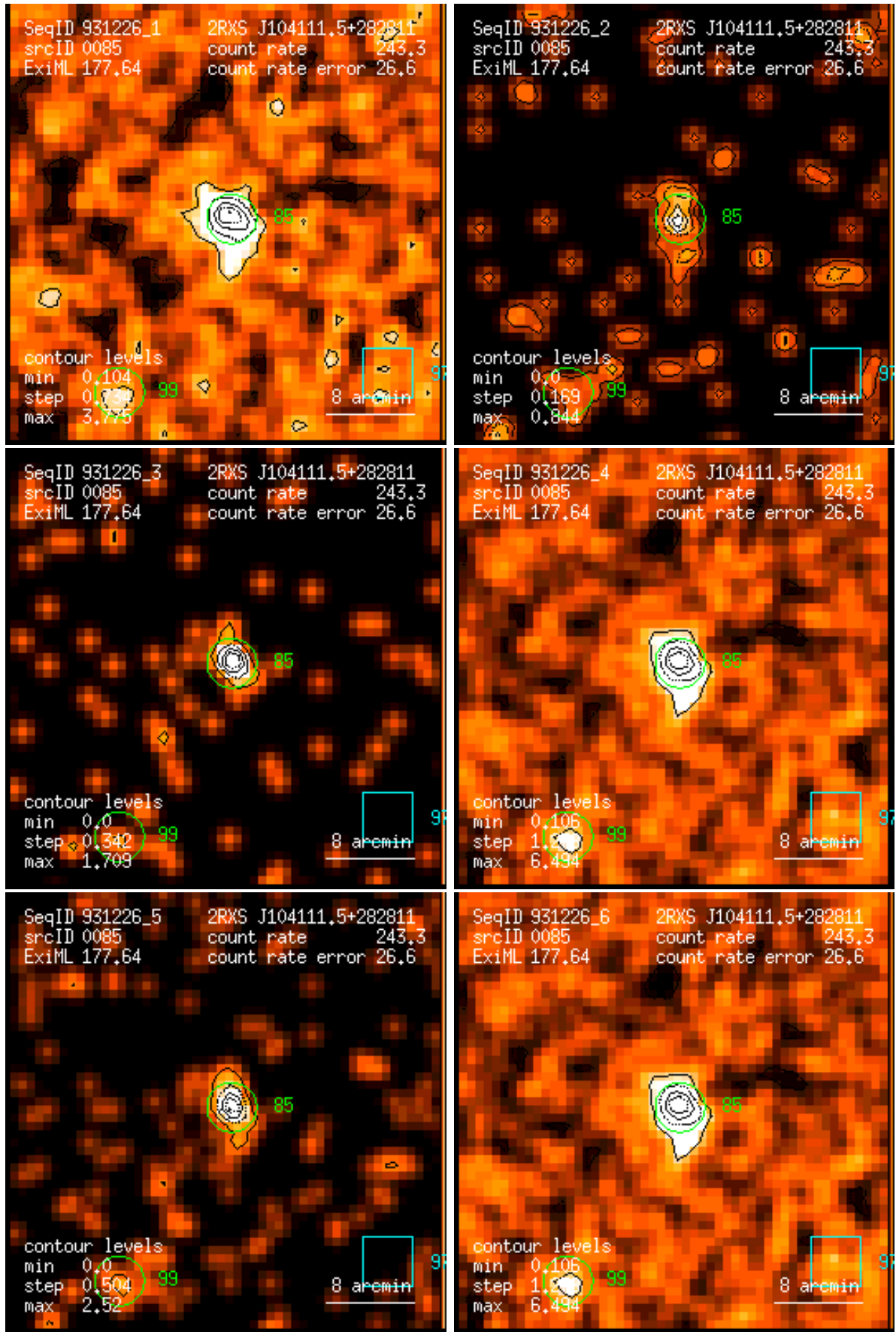
Figure 85: RASS 931226: detection 0085: band rate images, Gaussian filter: (1) PSPC channels 11 – 41, (2) 52 – 90, (3) 91 – 201, (4) 11 – 235, (5) 52 – 201, (6) 11 – 201. Broad band rates in counts/ks. Band rate contour levels in counts/ks/arcmin 2 .
