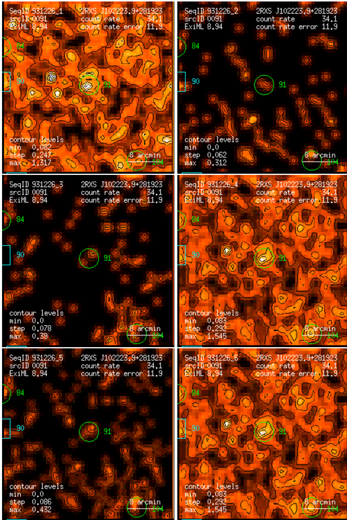
Figure 91: RASS 931226: detection 0091: band rate images, Gaussian filter: (1) PSPC channels 11 – 41, (2) 52 – 90, (3) 91 – 201, (4) 11 – 235, (5) 52 – 201, (6) 11 – 201. Broad band rates in counts/ks. Band rate contour levels in counts/ks/arcmin 2 .
