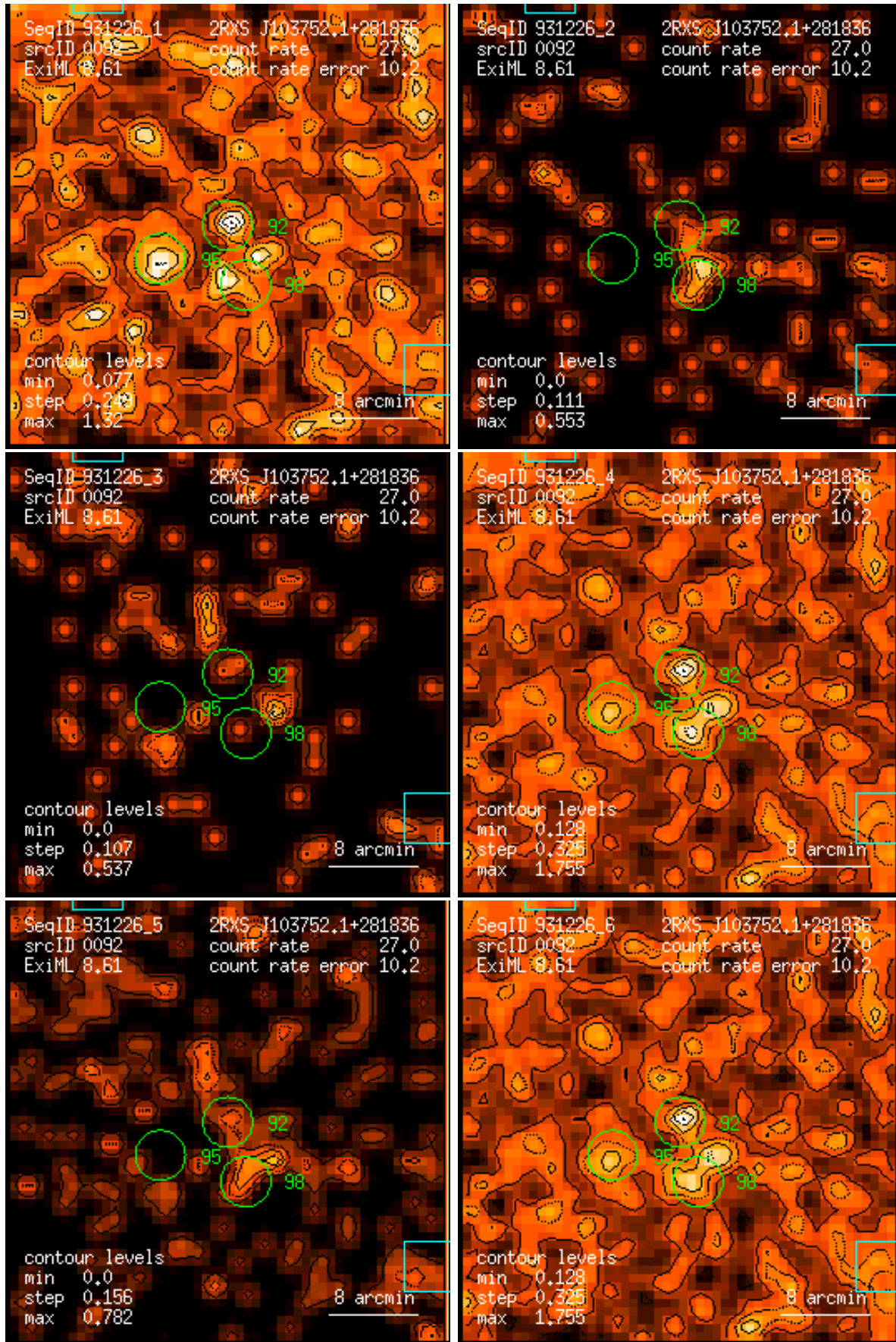
Figure 92: RASS 931226: detection 0092: band rate images, Gaussian filter: (1) PSPC channels 11 – 41, (2) 52 – 90, (3) 91 – 201, (4) 11 – 235, (5) 52 – 201, (6) 11 – 201. Broad band rates in counts/ks. Band rate contour levels in counts/ks/arcmin 2 .
