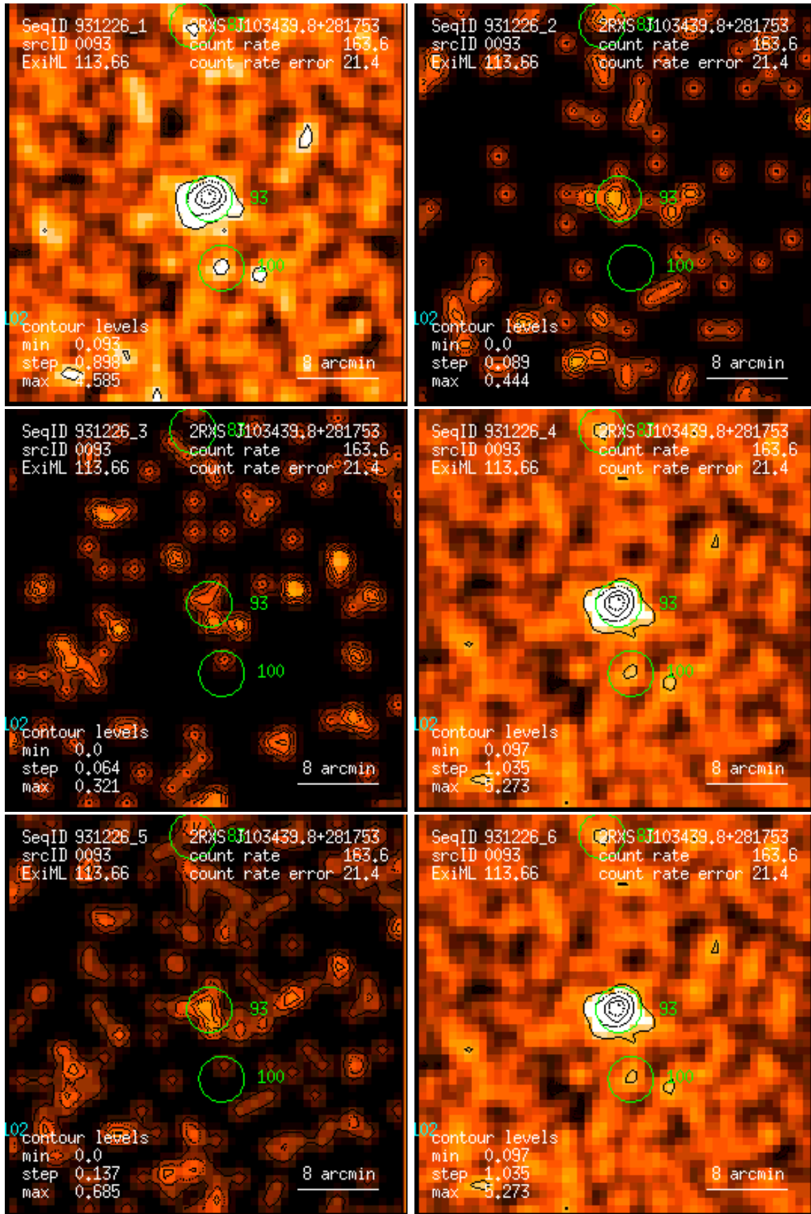
Figure 93: RASS 931226: detection 0093: band rate images, Gaussian filter: (1) PSPC channels 11 – 41, (2) 52 – 90, (3) 91 – 201, (4) 11 – 235, (5) 52 – 201, (6) 11 – 201. Broad band rates in counts/ks. Band rate contour levels in counts/ks/arcmin 2 .
