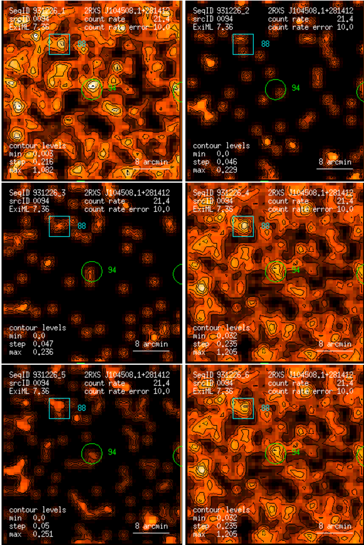
Figure 94: RASS 931226: detection 0094: band rate images, Gaussian filter: (1) PSPC channels 11 – 41, (2) 52 – 90, (3) 91 – 201, (4) 11 – 235, (5) 52 – 201, (6) 11 – 201. Broad band rates in counts/ks. Band rate contour levels in counts/ks/arcmin 2 .
