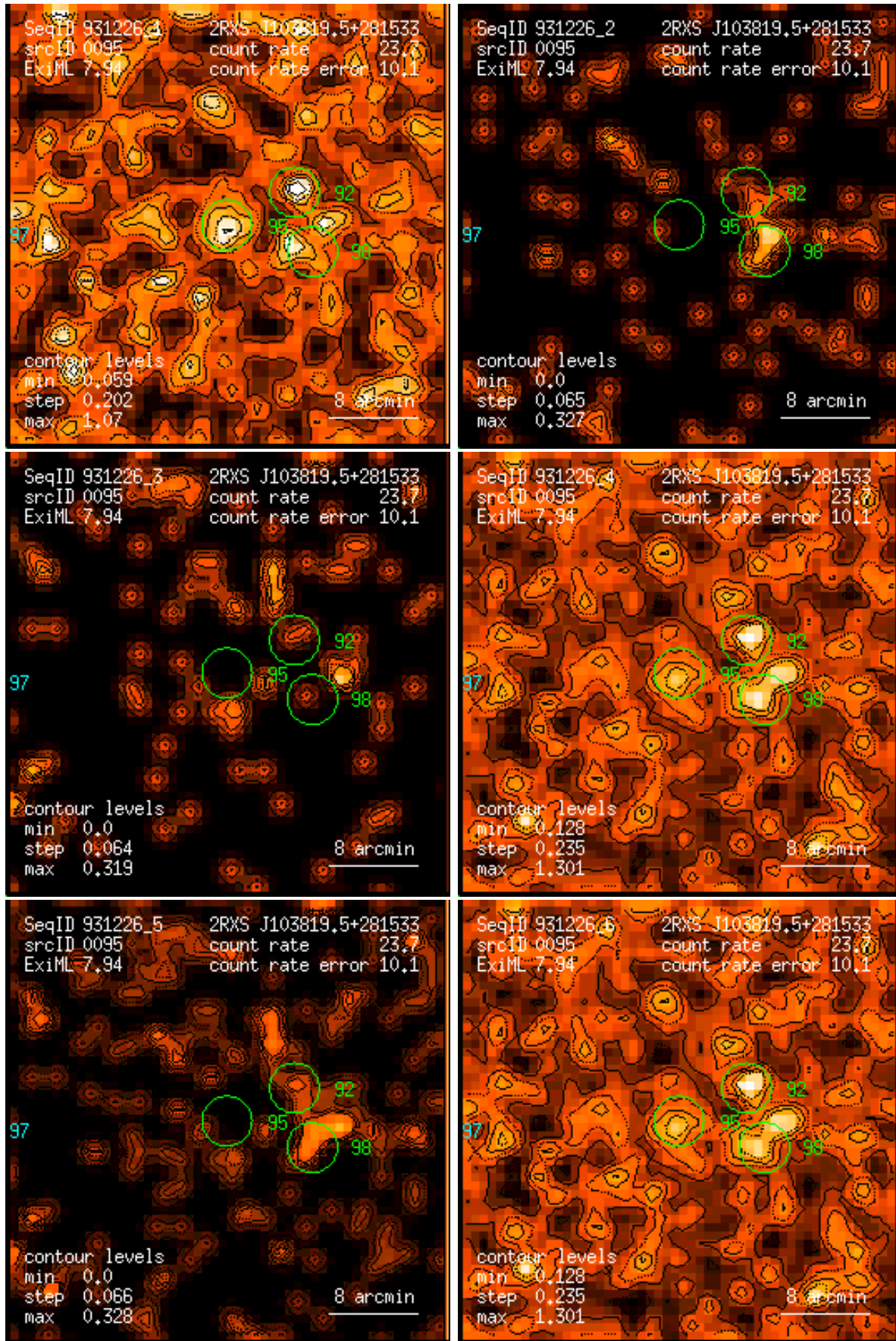
Figure 95: RASS 931226: detection 0095: band rate images, Gaussian filter: (1) PSPC channels 11 – 41, (2) 52 – 90, (3) 91 – 201, (4) 11 – 235, (5) 52 – 201, (6) 11 – 201. Broad band rates in counts/ks. Band rate contour levels in counts/ks/arcmin 2 .
