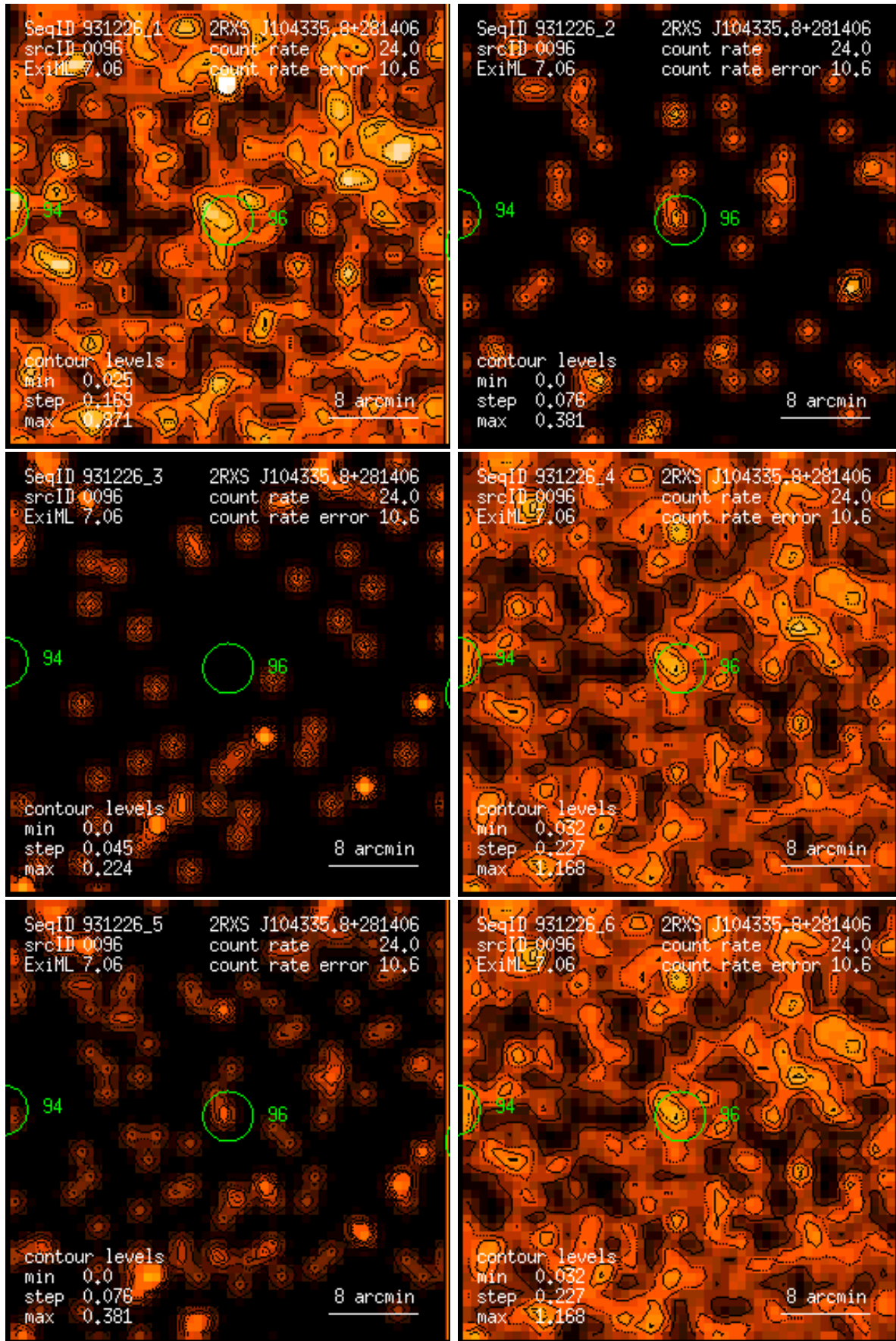
Figure 96: RASS 931226: detection 0096: band rate images, Gaussian filter: (1) PSPC channels 11 – 41, (2) 52 – 90, (3) 91 – 201, (4) 11 – 235, (5) 52 – 201, (6) 11 – 201. Broad band rates in counts/ks. Band rate contour levels in counts/ks/arcmin 2 .
