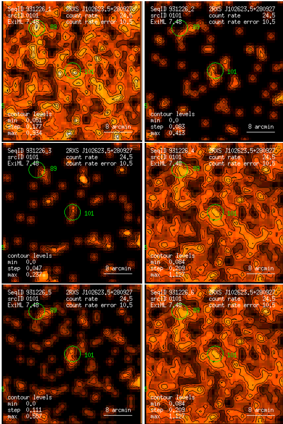
Figure 101: RASS 931226: detection 0101: band rate images, Gaussian filter: (1) PSPC channels 11 – 41, (2) 52 – 90, (3) 91 – 201, (4) 11 – 235, (5) 52 – 201, (6) 11 – 201. Broad band rates in counts/ks. Band rate contour levels in counts/ks/arcmin 2 .
