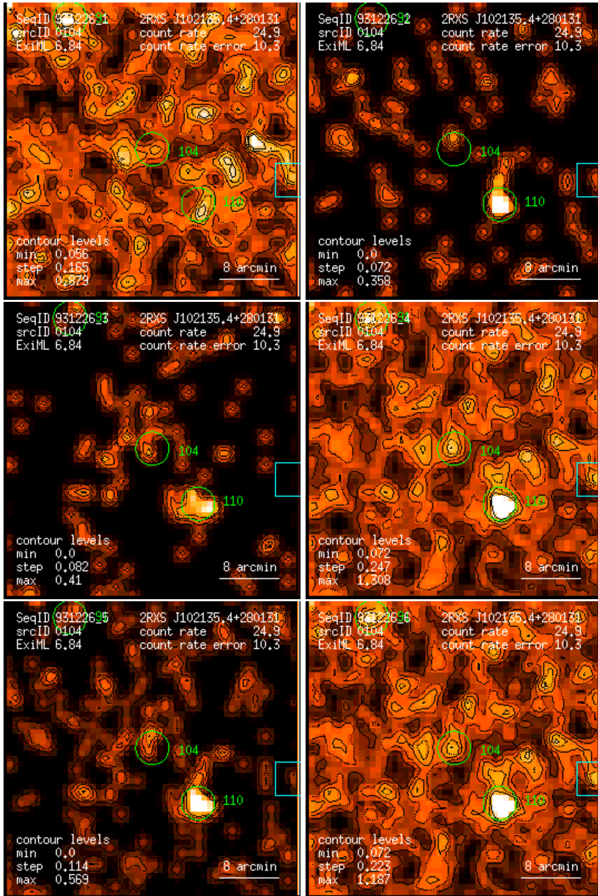
Figure 104: RASS 931226: detection 0104: band rate images, Gaussian filter: (1) PSPC channels 11 – 41, (2) 52 – 90, (3) 91 – 201, (4) 11 – 235, (5) 52 – 201, (6) 11 – 201. Broad band rates in counts/ks. Band rate contour levels in counts/ks/arcmin 2 .
