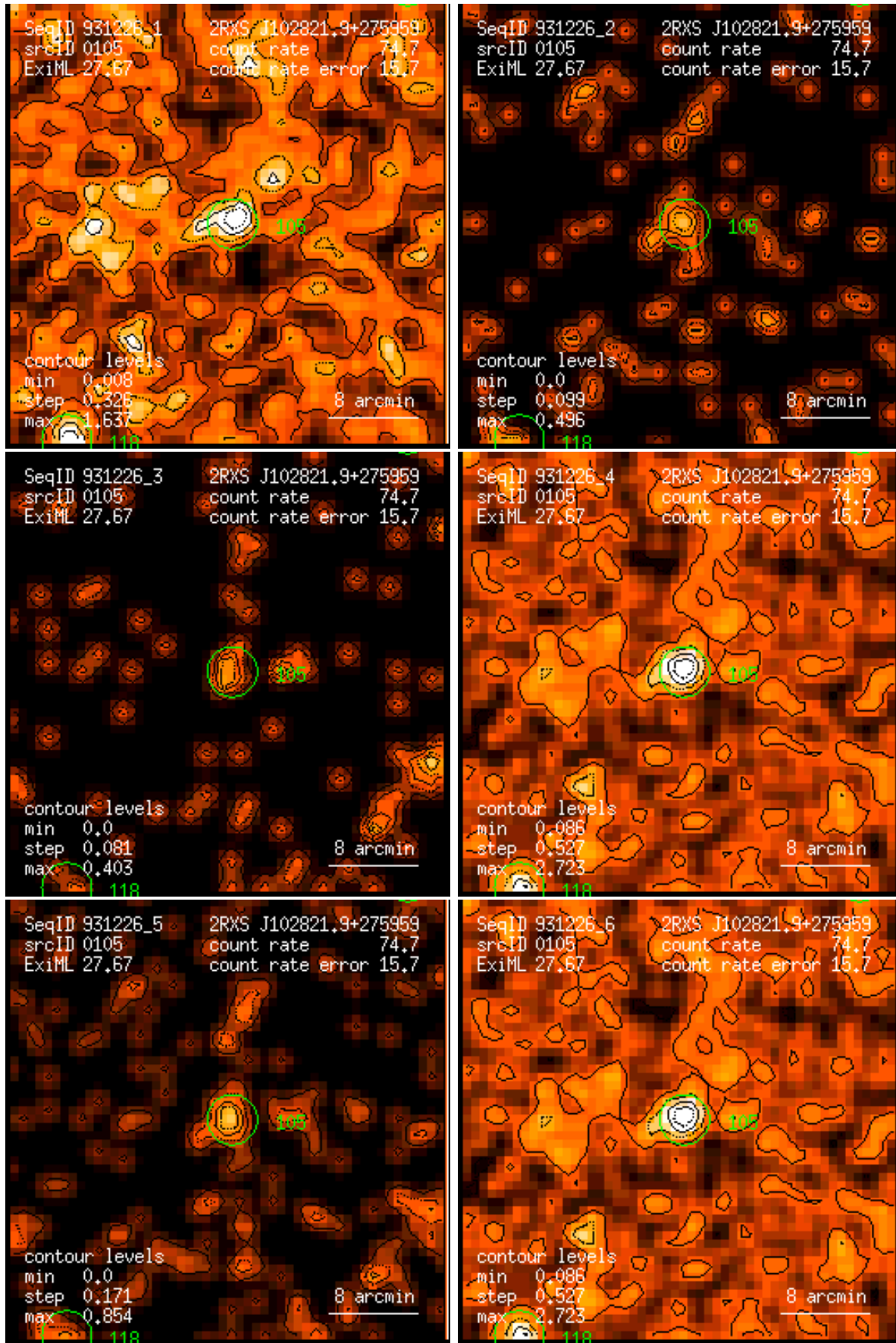
Figure 105: RASS 931226: detection 0105: band rate images, Gaussian filter: (1) PSPC channels 11 – 41, (2) 52 – 90, (3) 91 – 201, (4) 11 – 235, (5) 52 – 201, (6) 11 – 201. Broad band rates in counts/ks. Band rate contour levels in counts/ks/arcmin 2 .
