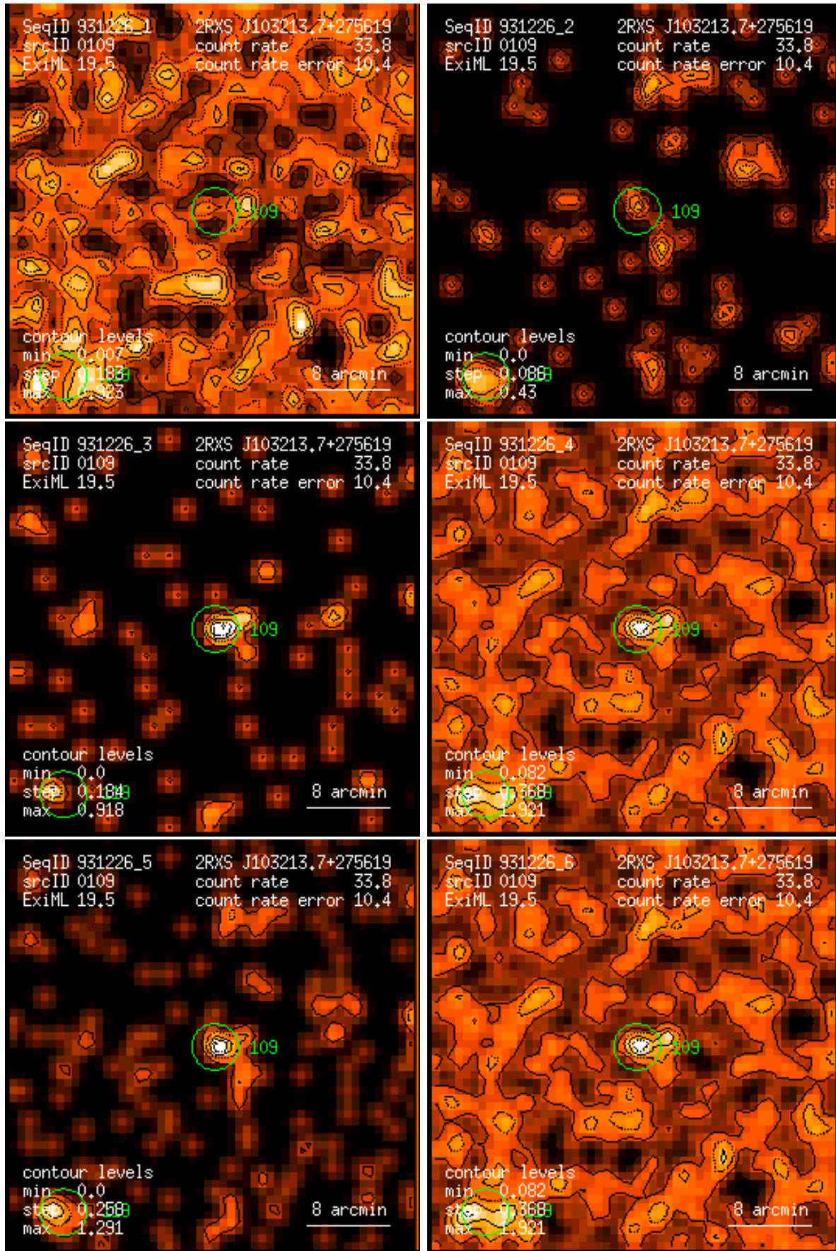
Figure 109: RASS 931226: detection 0109: band rate images, Gaussian filter: (1) PSPC channels 11 – 41, (2) 52 – 90, (3) 91 – 201, (4) 11 – 235, (5) 52 – 201, (6) 11 – 201. Broad band rates in counts/ks. Band rate contour levels in counts/ks/arcmin 2 .
