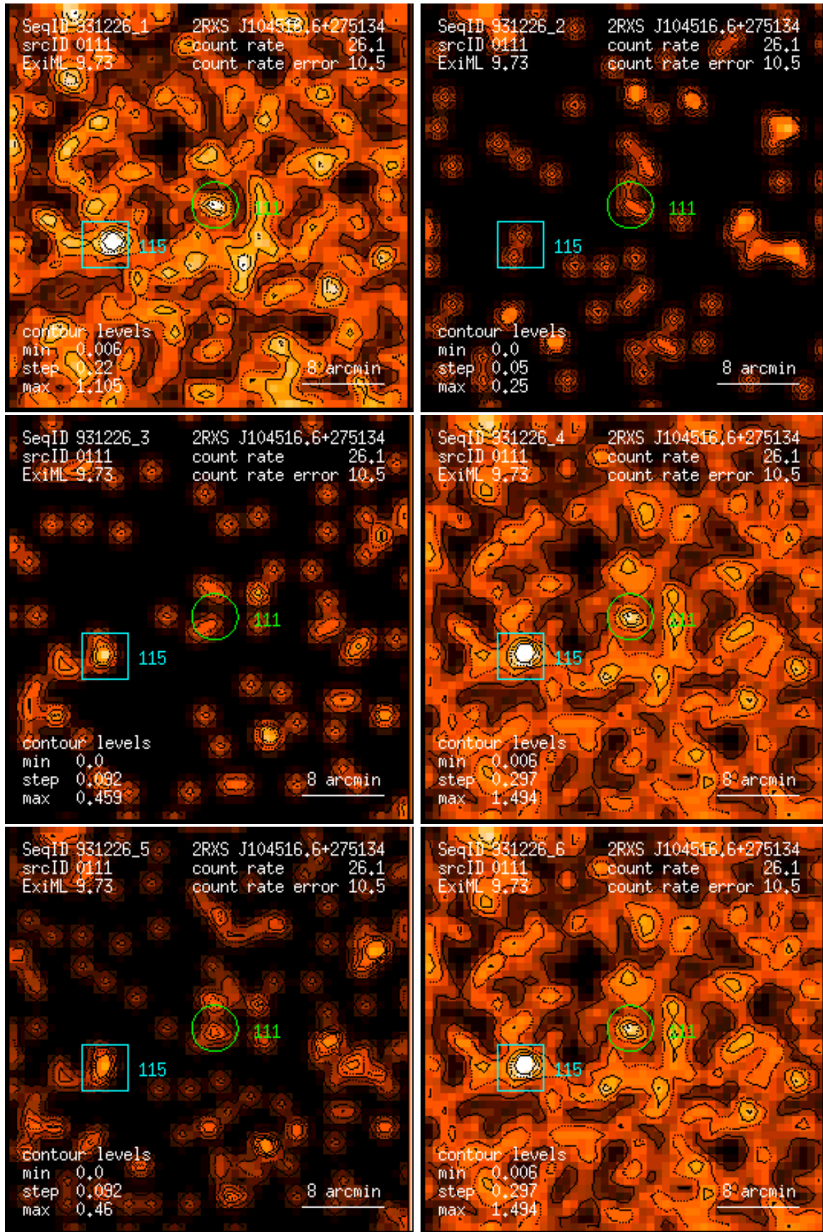
Figure 111: RASS 931226: detection 0111: band rate images, Gaussian filter: (1) PSPC channels 11 – 41, (2) 52 – 90, (3) 91 – 201, (4) 11 – 235, (5) 52 – 201, (6) 11 – 201. Broad band rates in counts/ks. Band rate contour levels in counts/ks/arcmin 2 .
