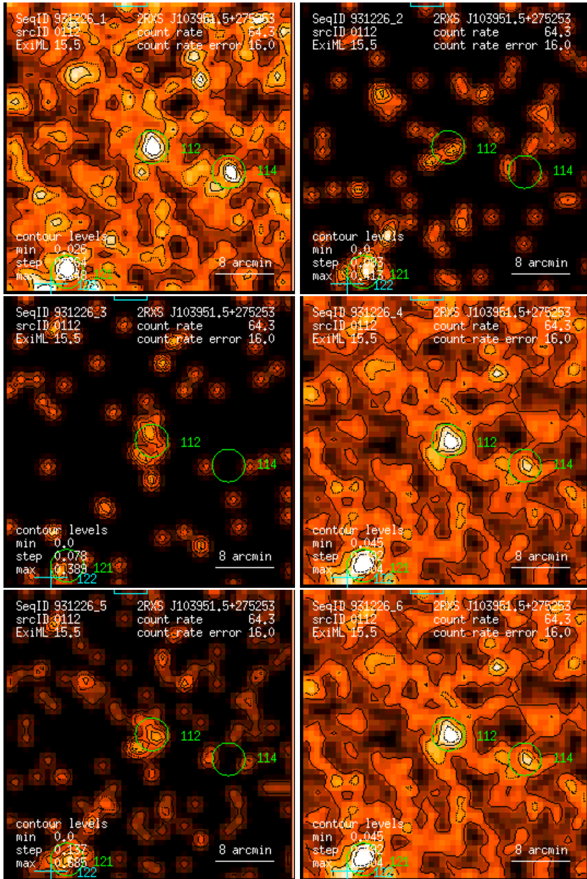
Figure 112: RASS 931226: detection 0112: band rate images, Gaussian filter: (1) PSPC channels 11 – 41, (2) 52 – 90, (3) 91 – 201, (4) 11 – 235, (5) 52 – 201, (6) 11 – 201. Broad band rates in counts/ks. Band rate contour levels in counts/ks/arcmin 2 .
