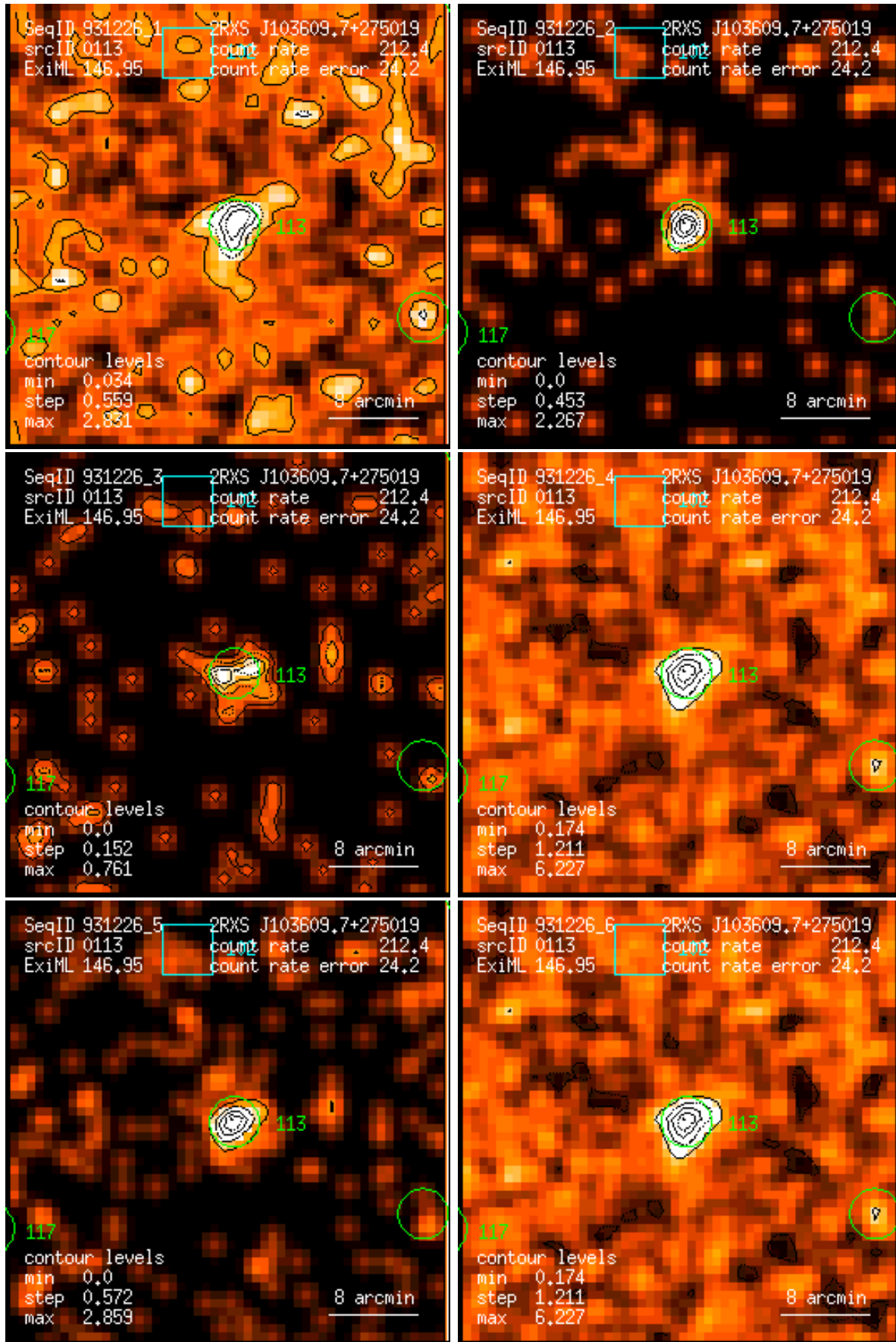
Figure 113: RASS 931226: detection 0113: band rate images, Gaussian filter: (1) PSPC channels 11 – 41, (2) 52 – 90, (3) 91 – 201, (4) 11 – 235, (5) 52 – 201, (6) 11 – 201. Broad band rates in counts/ks. Band rate contour levels in counts/ks/arcmin 2 .
