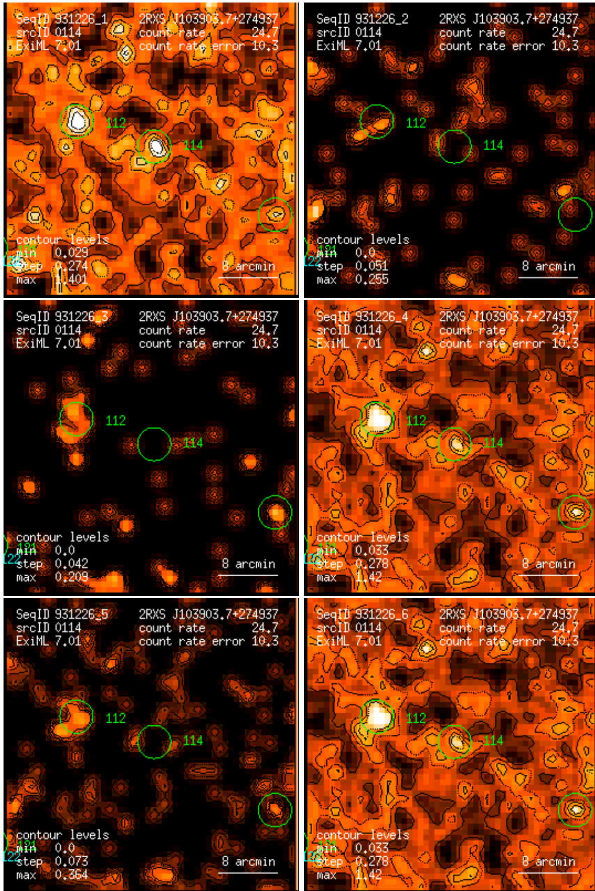
Figure 114: RASS 931226: detection 0114: band rate images, Gaussian filter: (1) PSPC channels 11 – 41, (2) 52 – 90, (3) 91 – 201, (4) 11 – 235, (5) 52 – 201, (6) 11 – 201. Broad band rates in counts/ks. Band rate contour levels in counts/ks/arcmin 2 .
