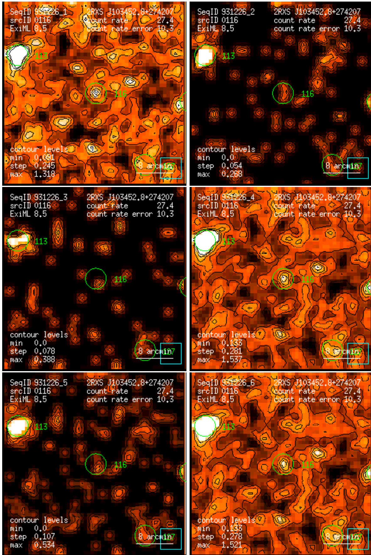
Figure 116: RASS 931226: detection 0116: band rate images, Gaussian filter: (1) PSPC channels 11 – 41, (2) 52 – 90, (3) 91 – 201, (4) 11 – 235, (5) 52 – 201, (6) 11 – 201. Broad band rates in counts/ks. Band rate contour levels in counts/ks/arcmin 2 .
