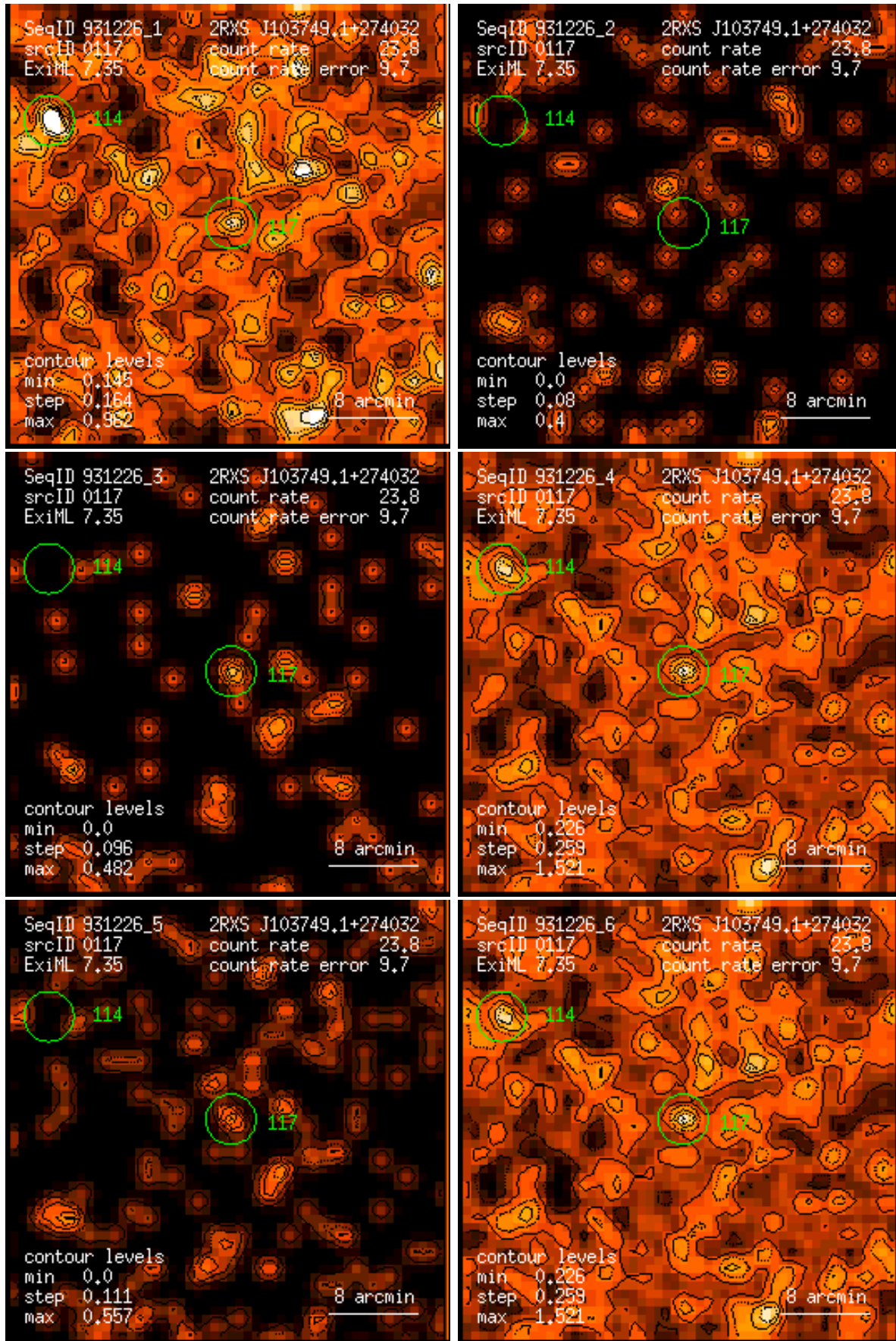
Figure 117: RASS 931226: detection 0117: band rate images, Gaussian filter: (1) PSPC channels 11 – 41, (2) 52 – 90, (3) 91 – 201, (4) 11 – 235, (5) 52 – 201, (6) 11 – 201. Broad band rates in counts/ks. Band rate contour levels in counts/ks/arcmin 2 .
