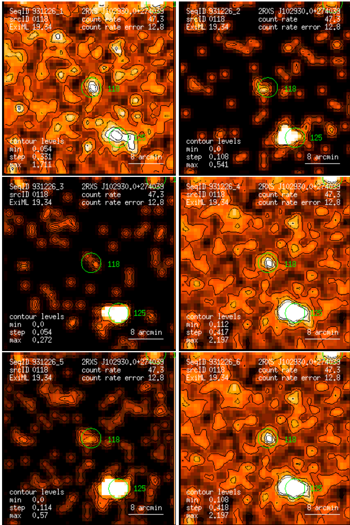
Figure 118: RASS 931226: detection 0118: band rate images, Gaussian filter: (1) PSPC channels 11 – 41, (2) 52 – 90, (3) 91 – 201, (4) 11 – 235, (5) 52 – 201, (6) 11 – 201. Broad band rates in counts/ks. Band rate contour levels in counts/ks/arcmin 2 .
