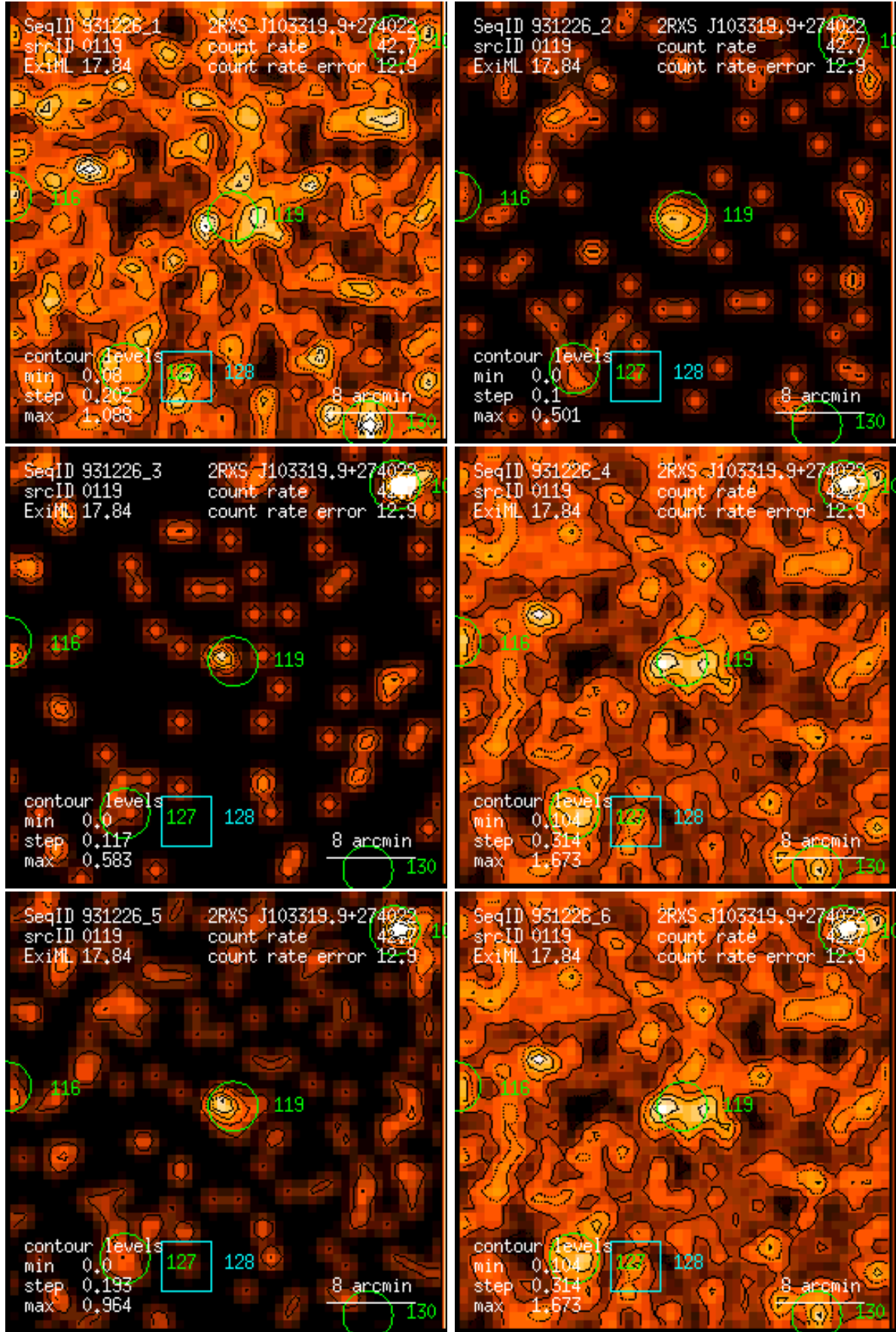
Figure 119: RASS 931226: detection 0119: band rate images, Gaussian filter: (1) PSPC channels 11 – 41, (2) 52 – 90, (3) 91 – 201, (4) 11 – 235, (5) 52 – 201, (6) 11 – 201. Broad band rates in counts/ks. Band rate contour levels in counts/ks/arcmin 2 .
